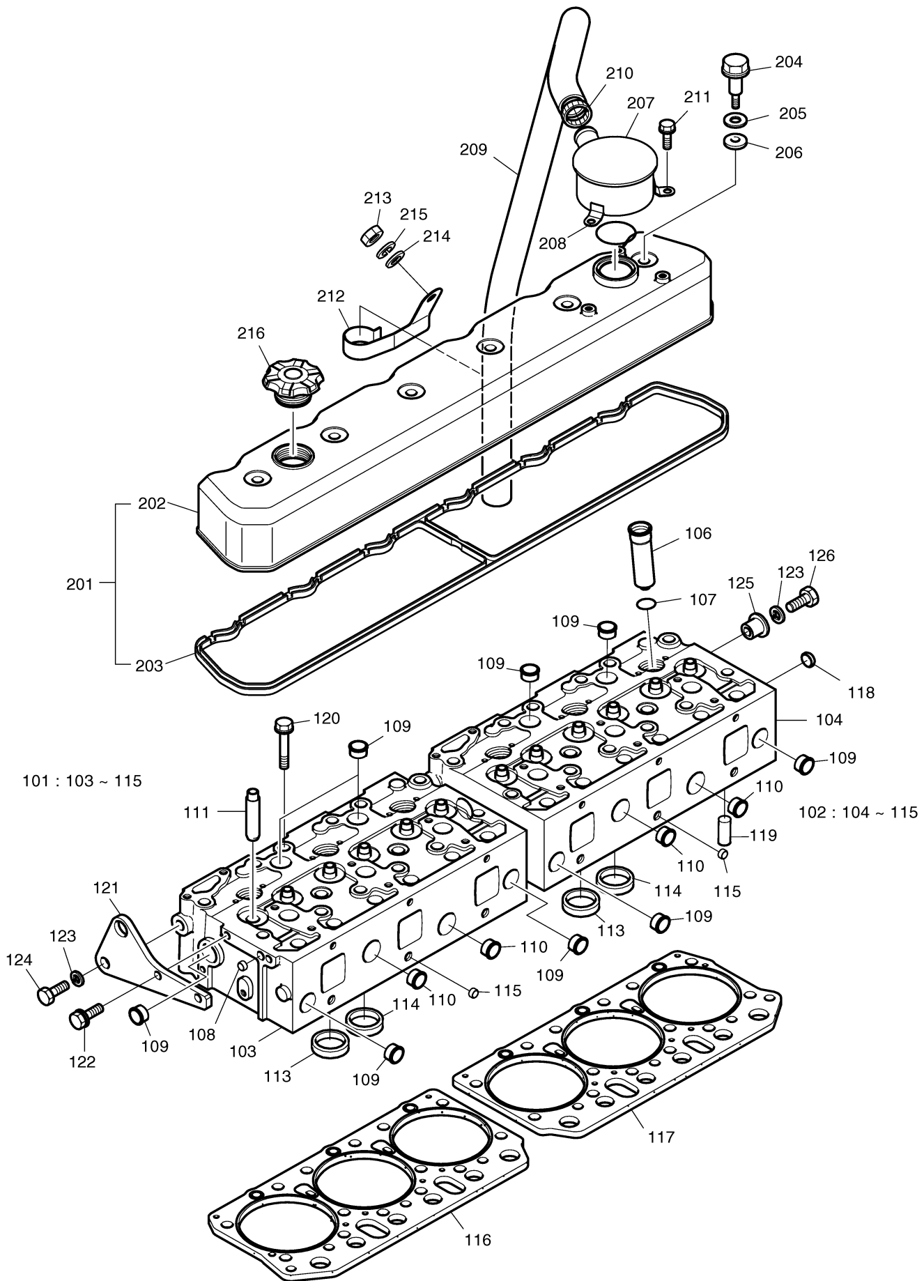
Fig. 017 CYLINDER HEAD
