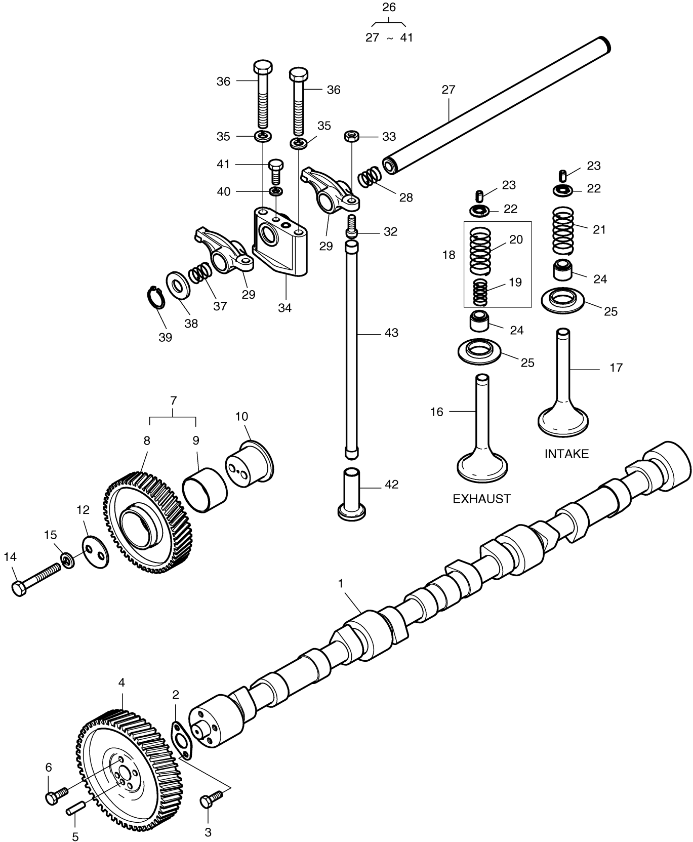
Fig. 018 ENGINE TIMING
