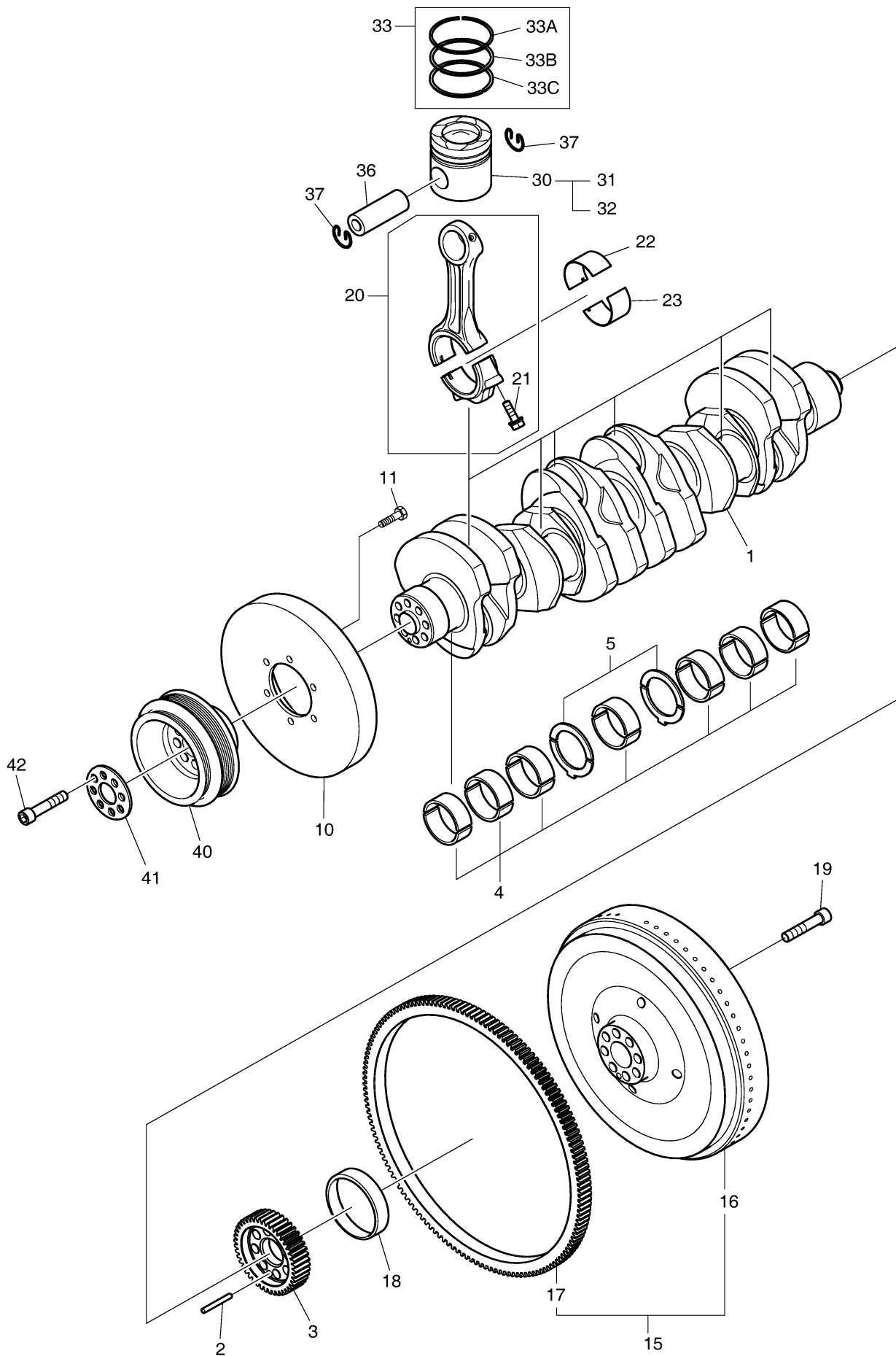
Fig. 016 DRIVING SYSTEM
