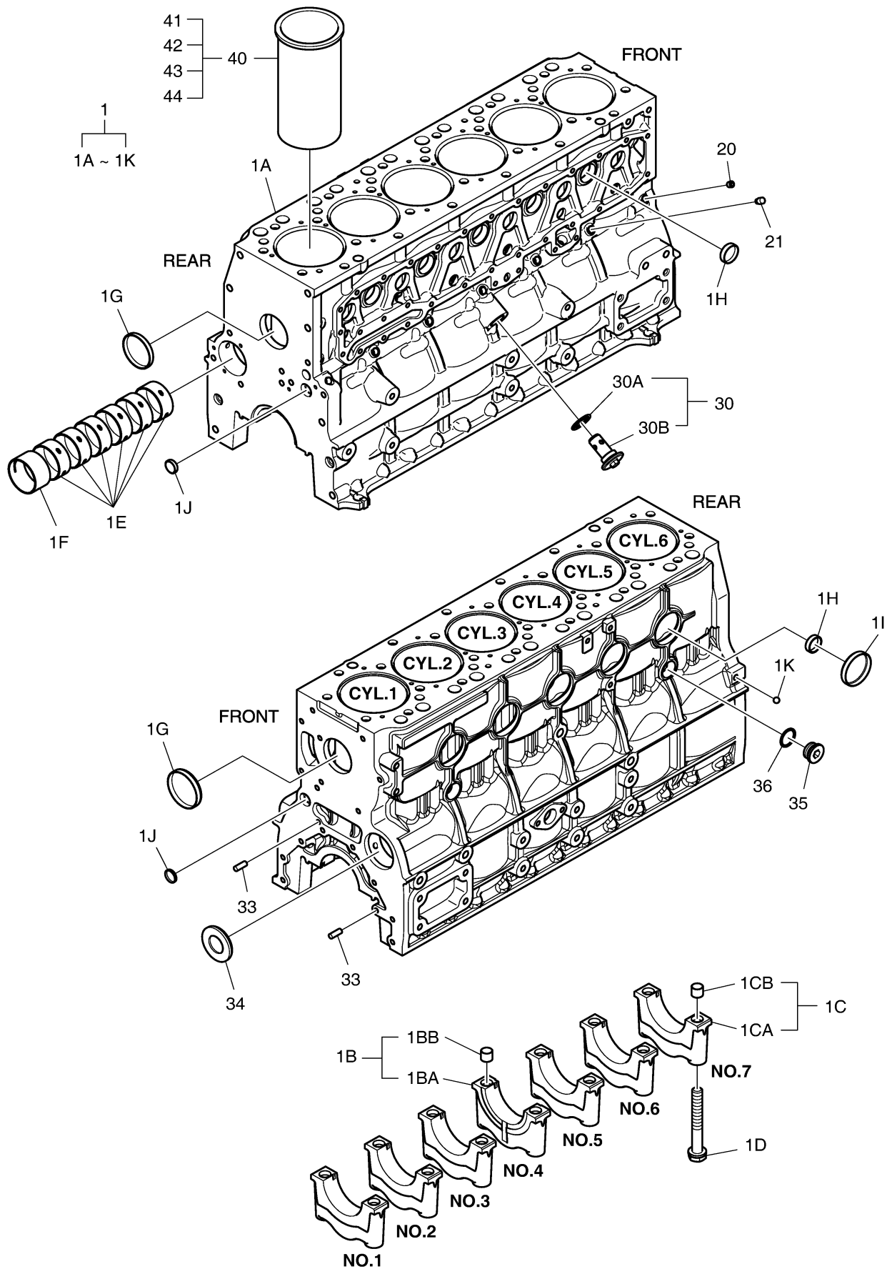
Fig. 001 CYLINDER BLOCK
