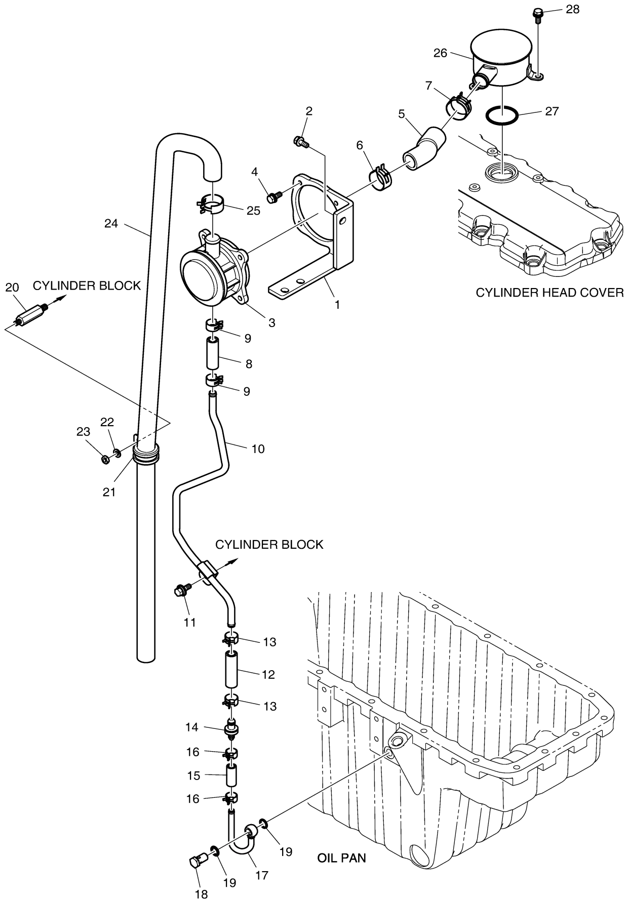
Fig. 006 BREATHER SYSTEM
