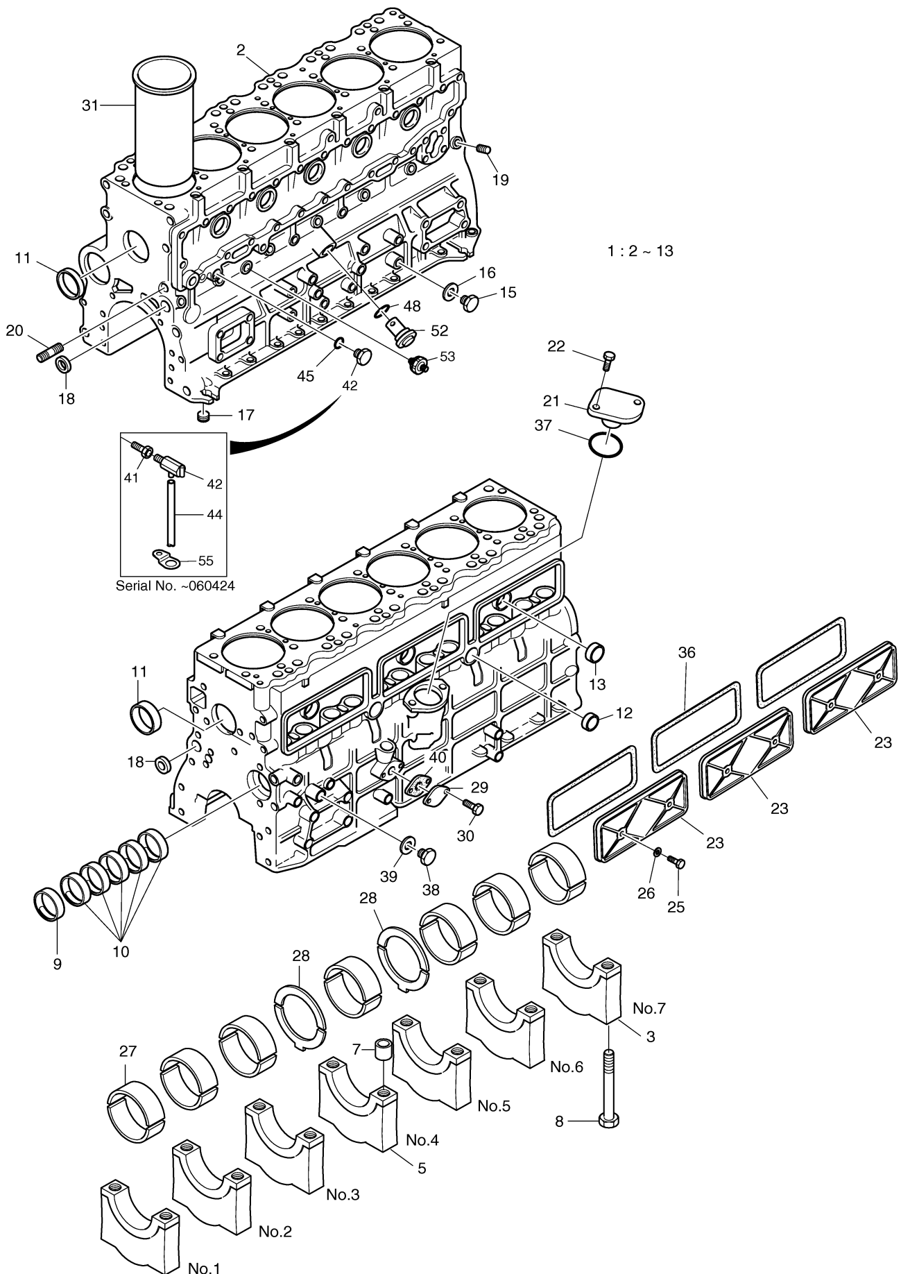
Fig. 001 CYLINDER BLOCK [2001 ~ 2016]
