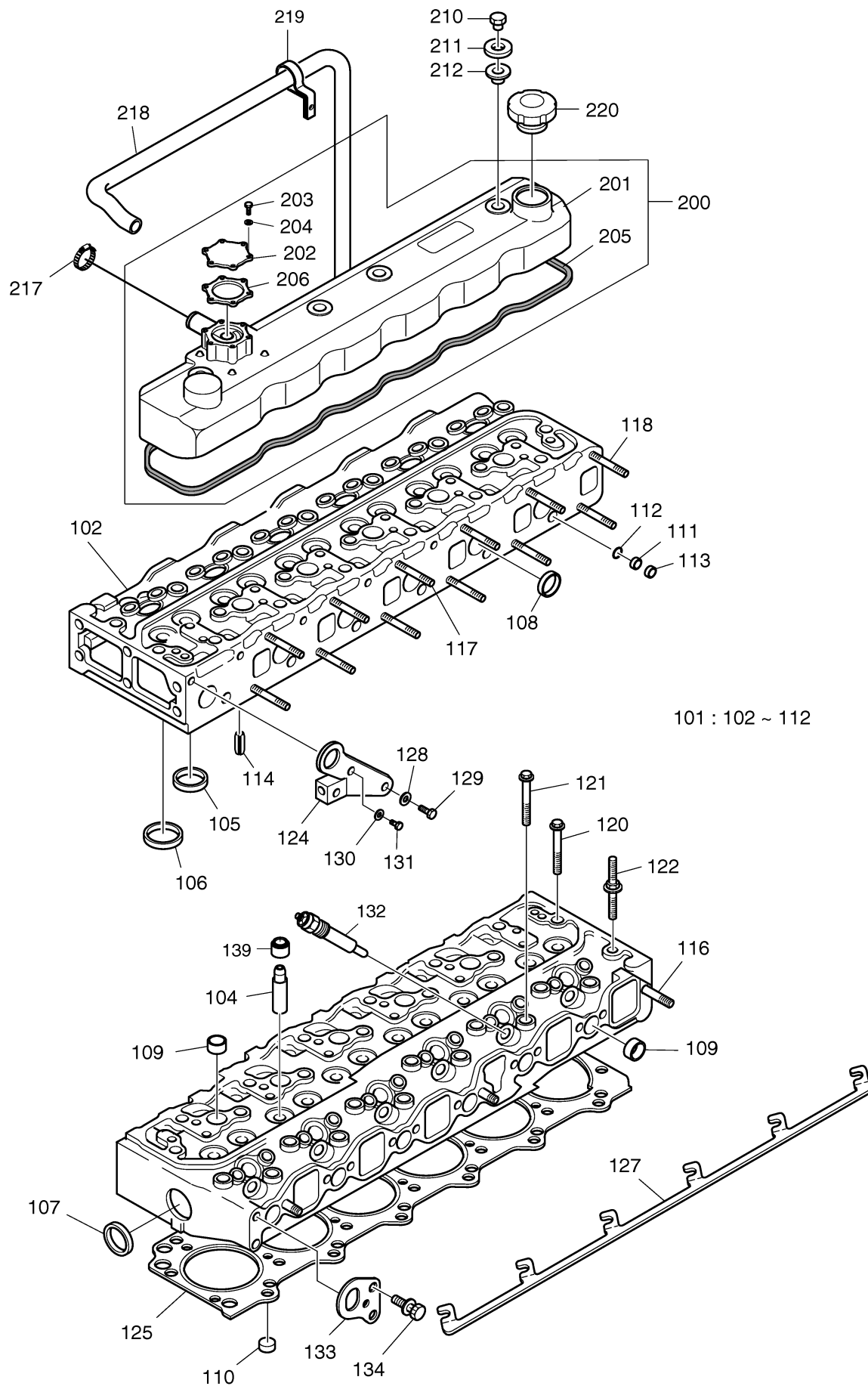
Fig. 005 CYLINDER HEAD [2001 ~ 2016]
