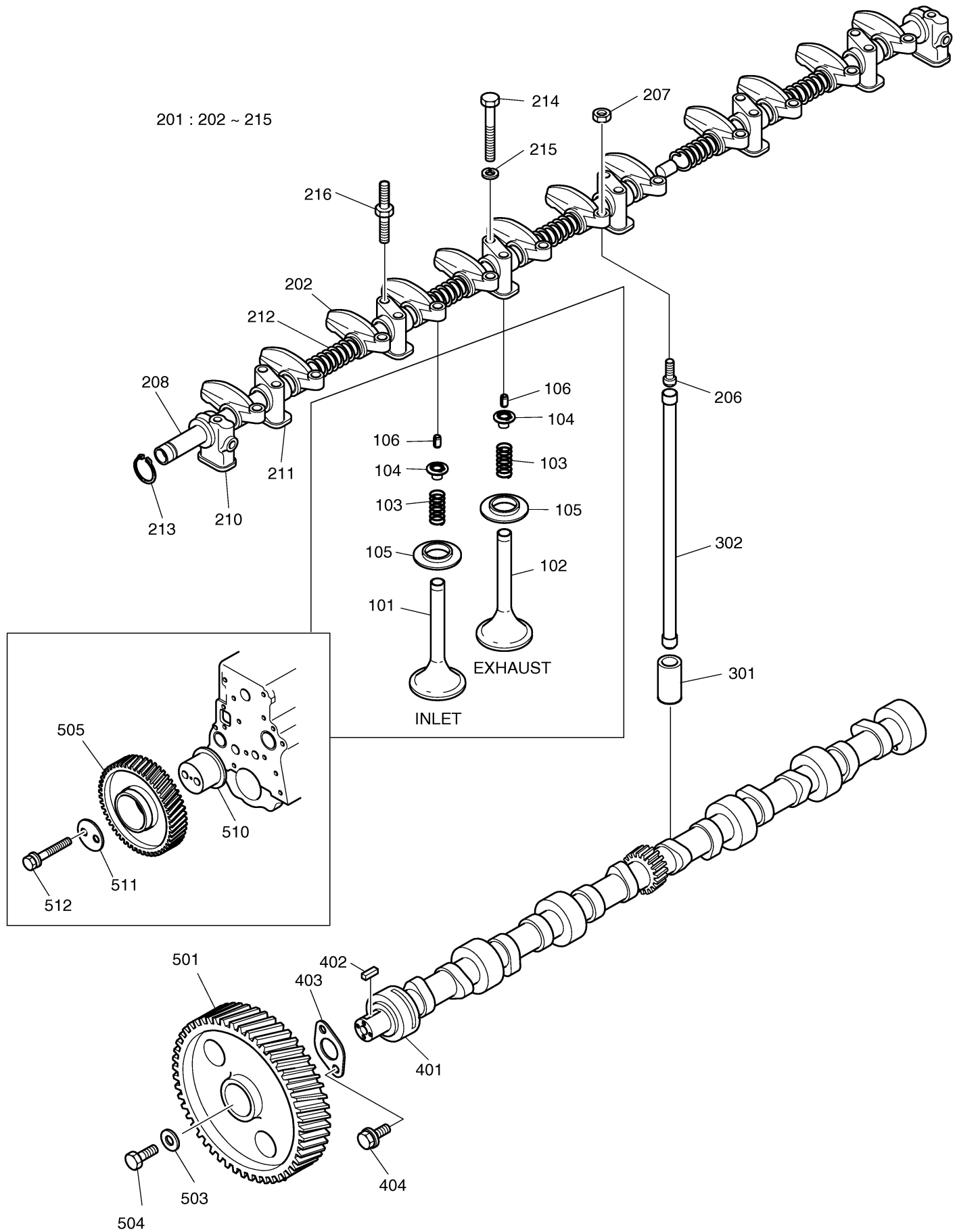
Fig. 006 VALVE MECHANISM [2001 ~
