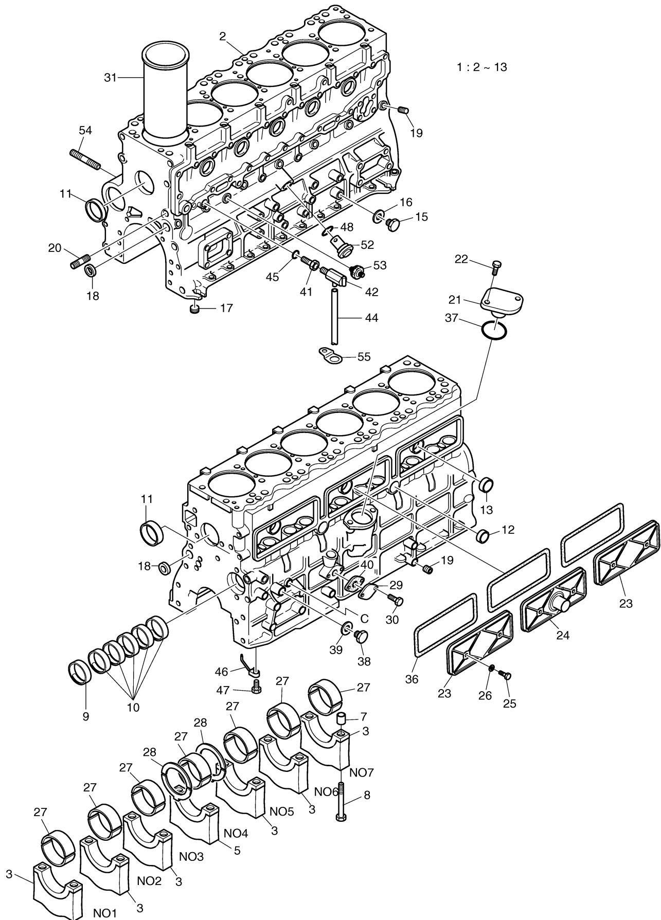
Fig. 001 CYLINDER BLOCK
