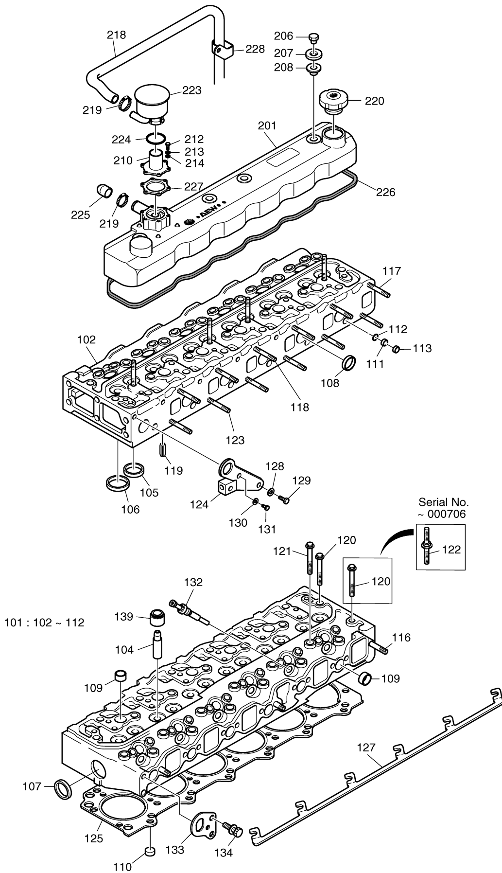
Fig. 005 CYLINDER HEAD
