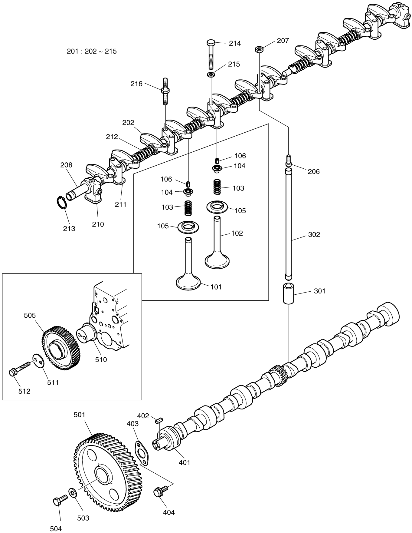
Fig. 006 VALVE MECHANISM
