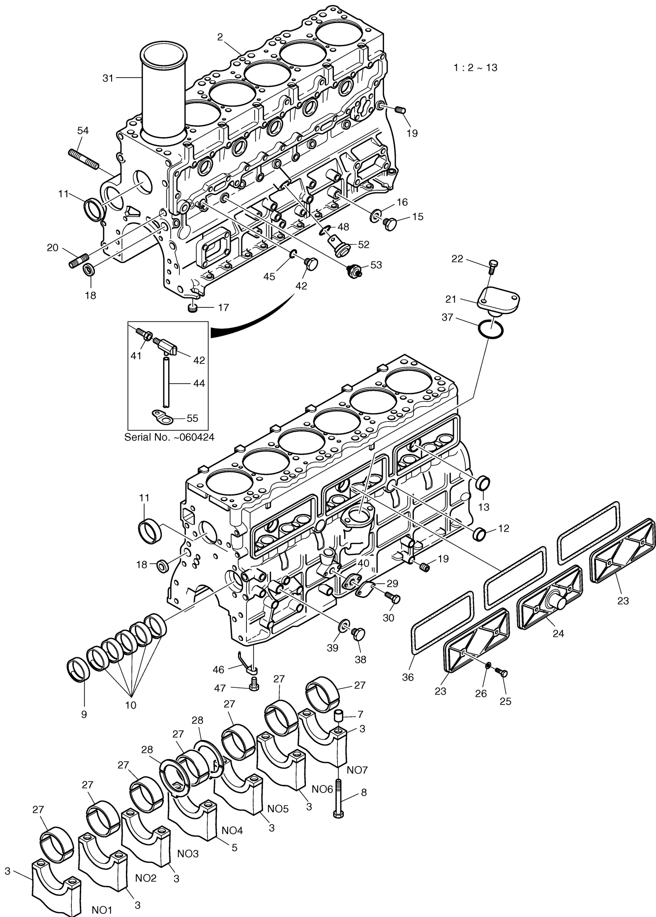
Fig. 001 CYLINDER BLOCK
