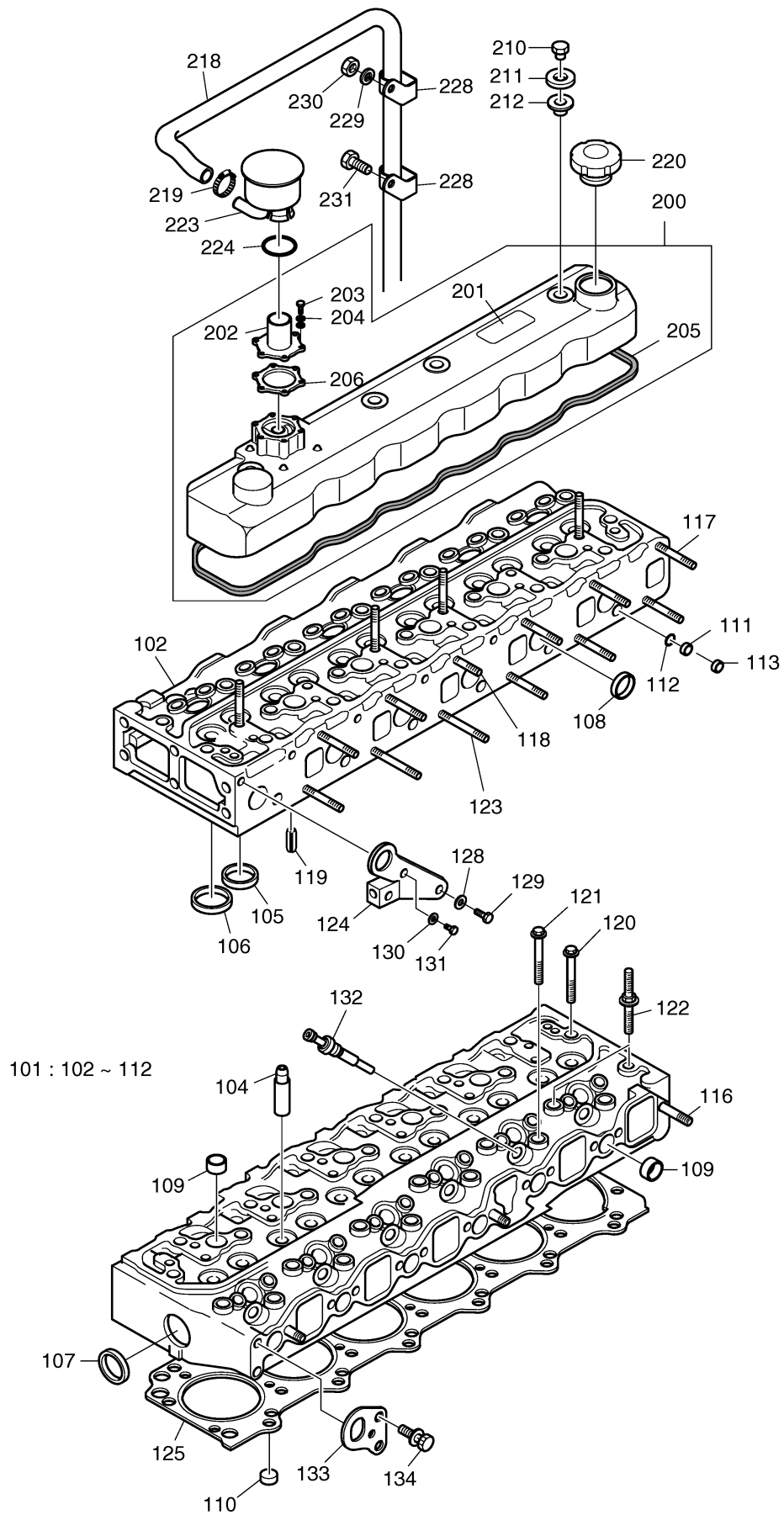
Fig. 005 CYLINDER HEAD
