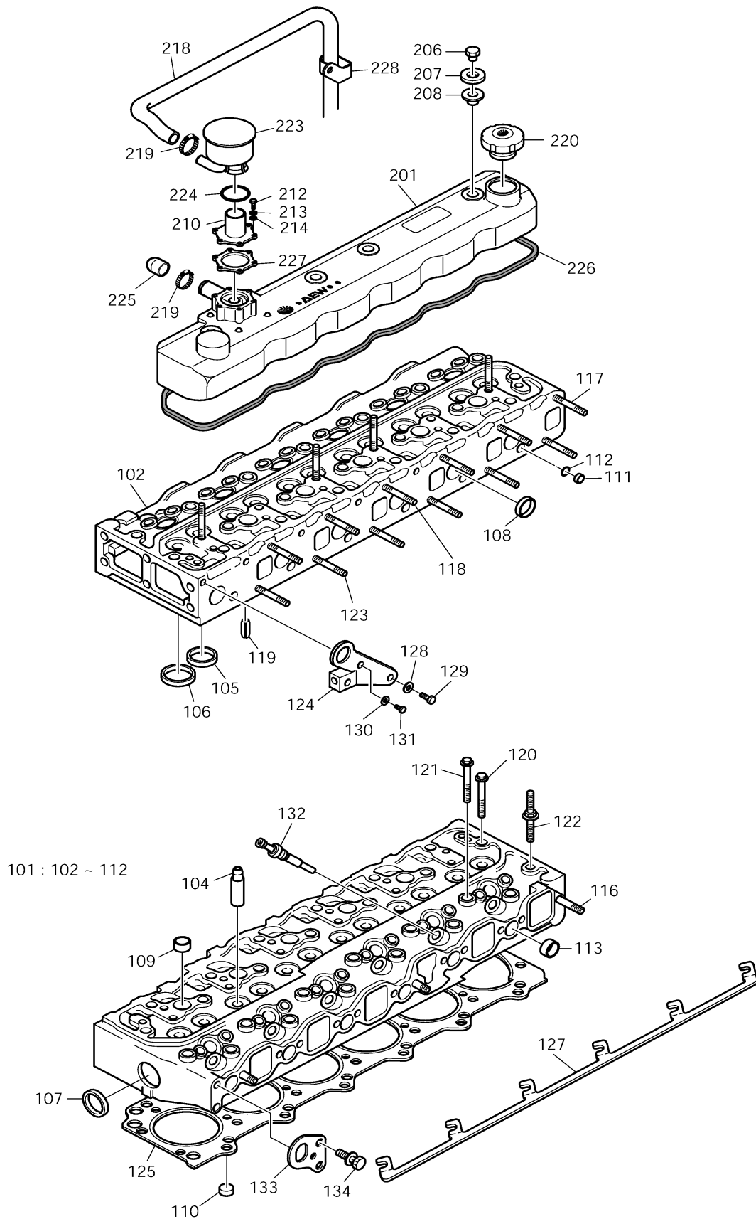
Fig. 005 CYLINDER HEAD
