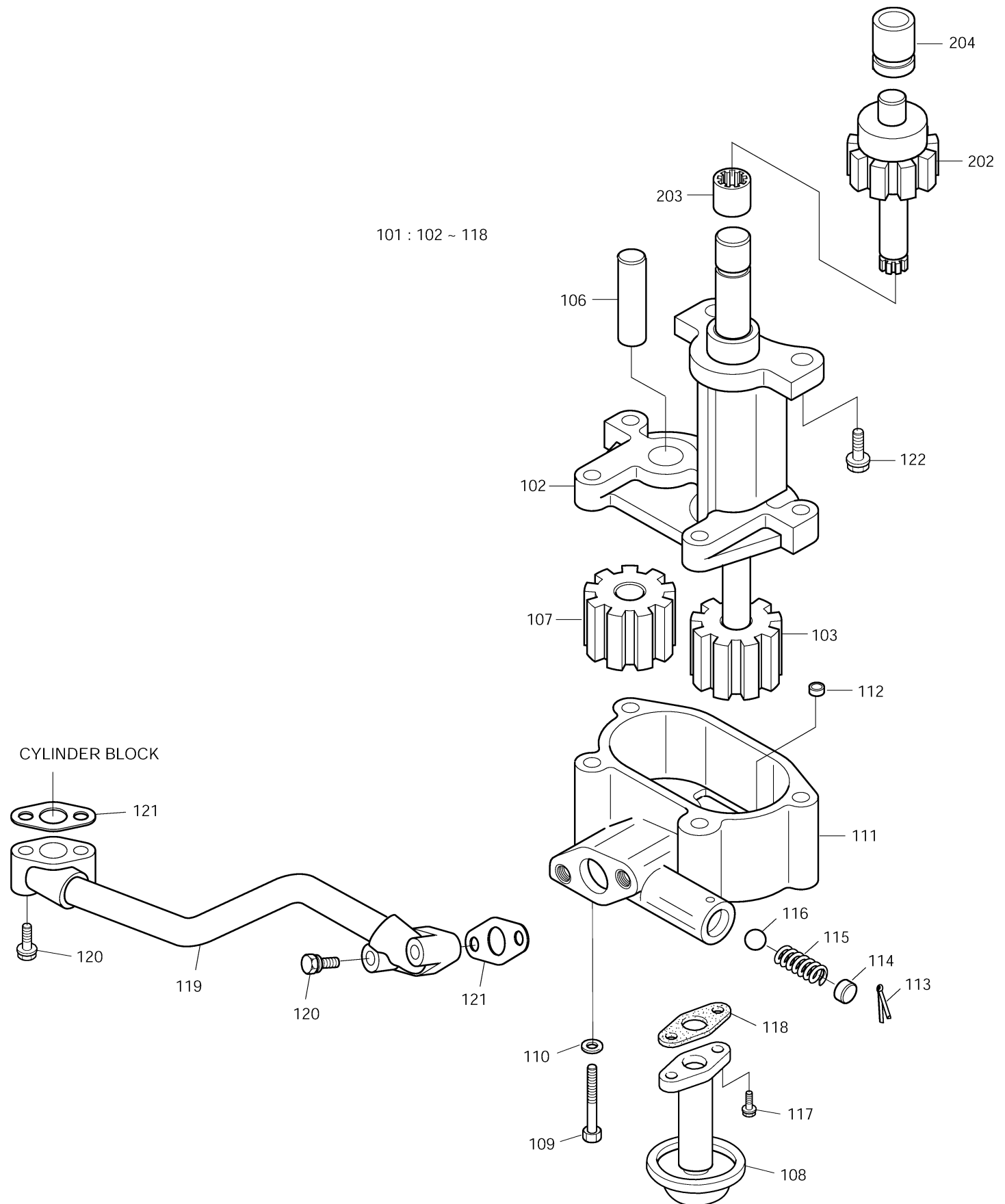
Fig. 007 OIL PUMP
