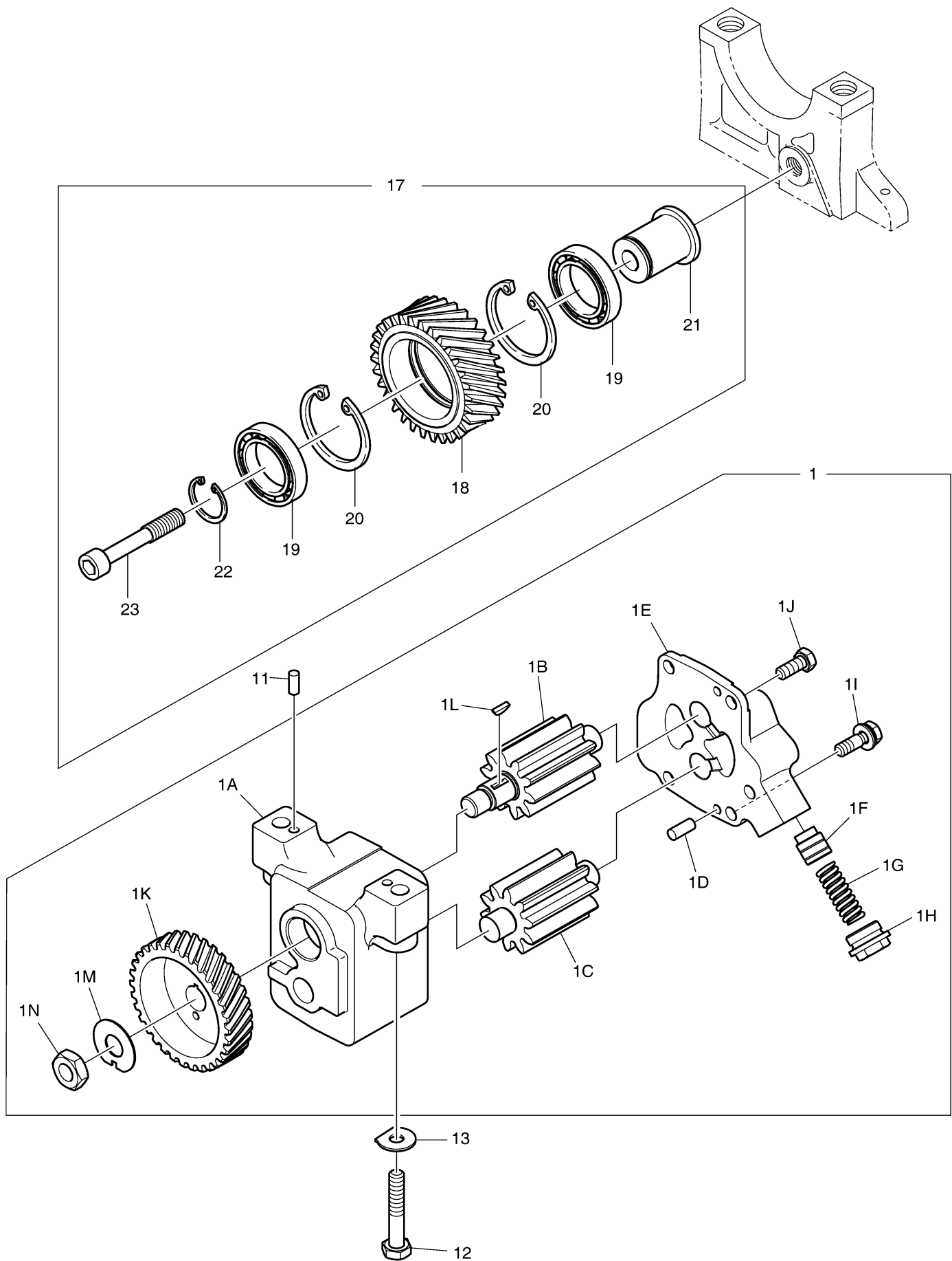
Fig. 008 OIL PUMP
