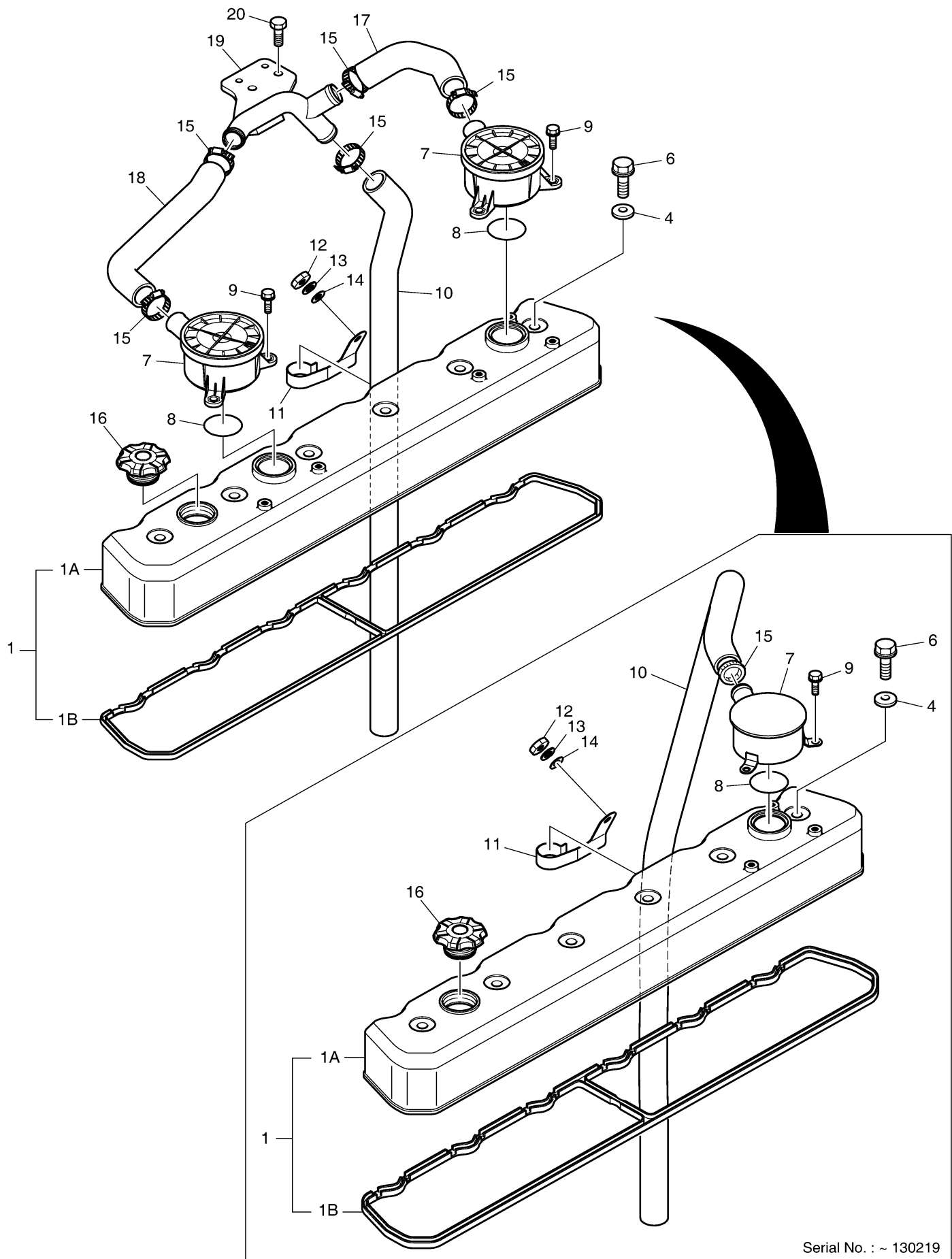
Fig. 006 CYLINDER HEAD COVER
