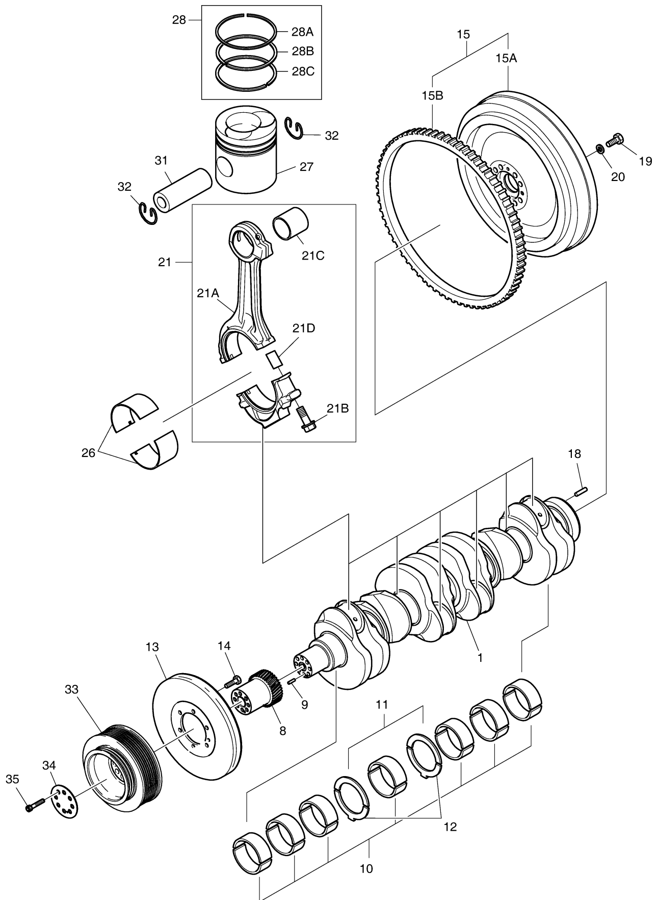
Fig. 004 DRIVING SYSTEM
