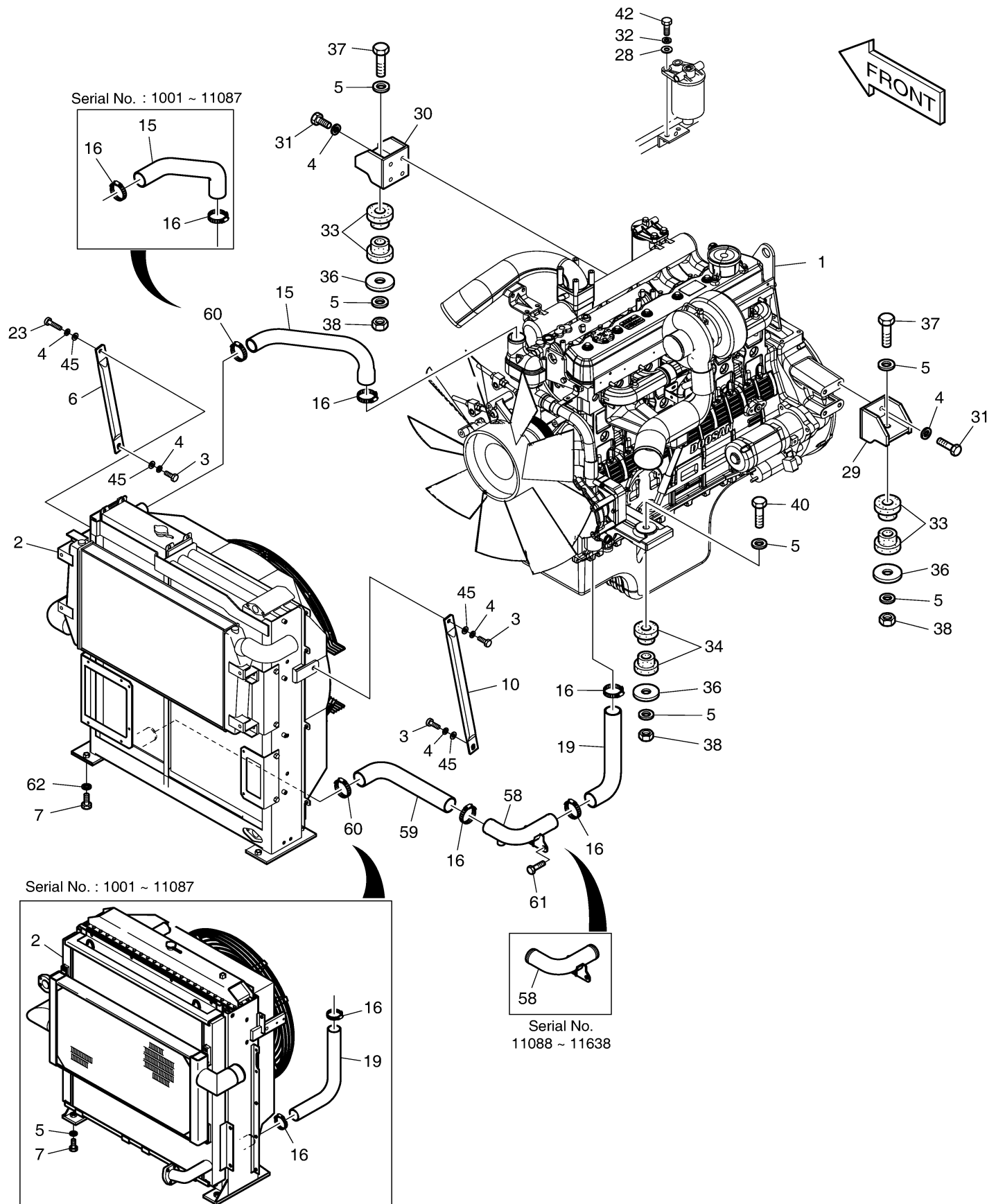
Fig. 1120 ENGINE MOUNTING
