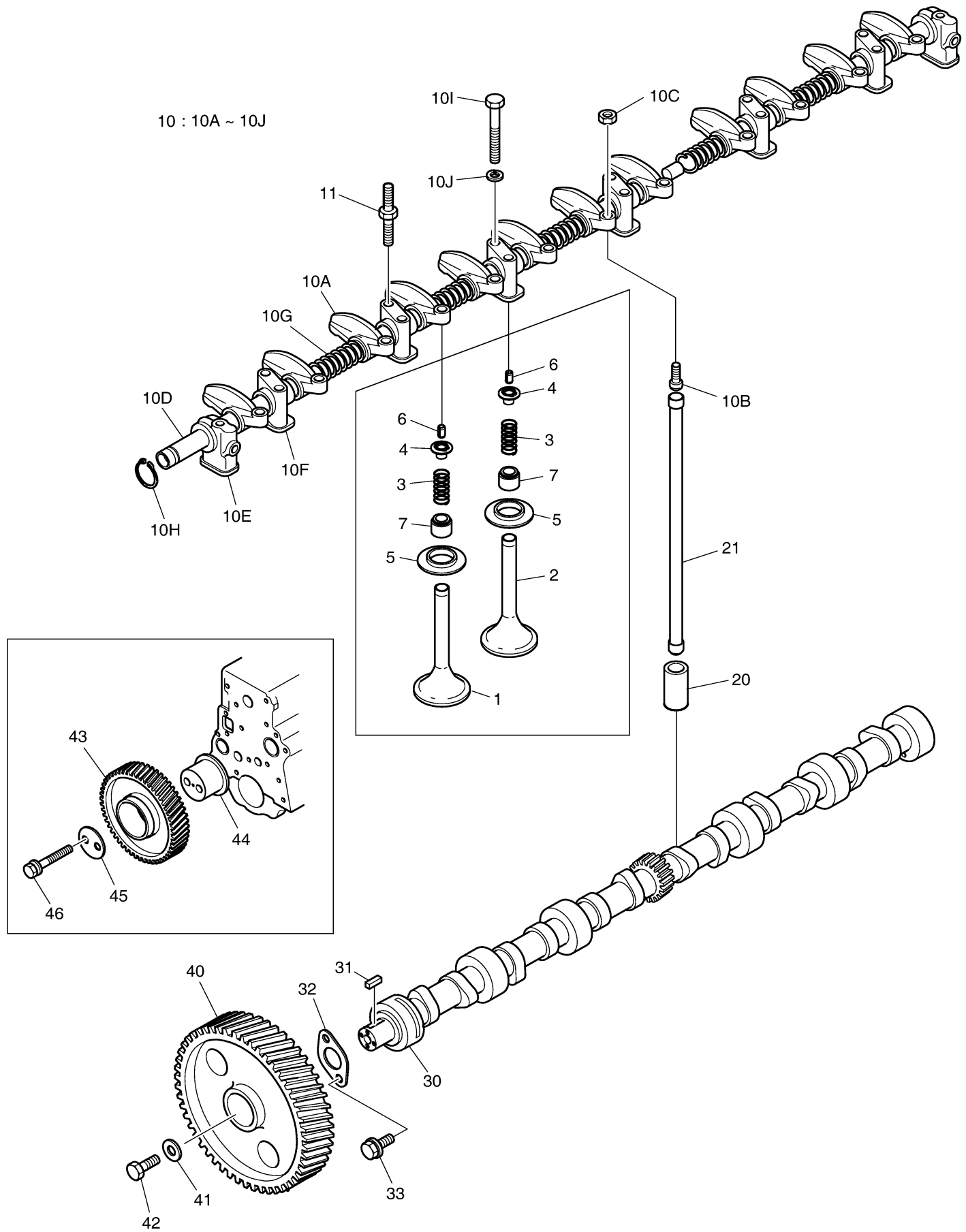
Fig. 006 VALVE MECHANISM
