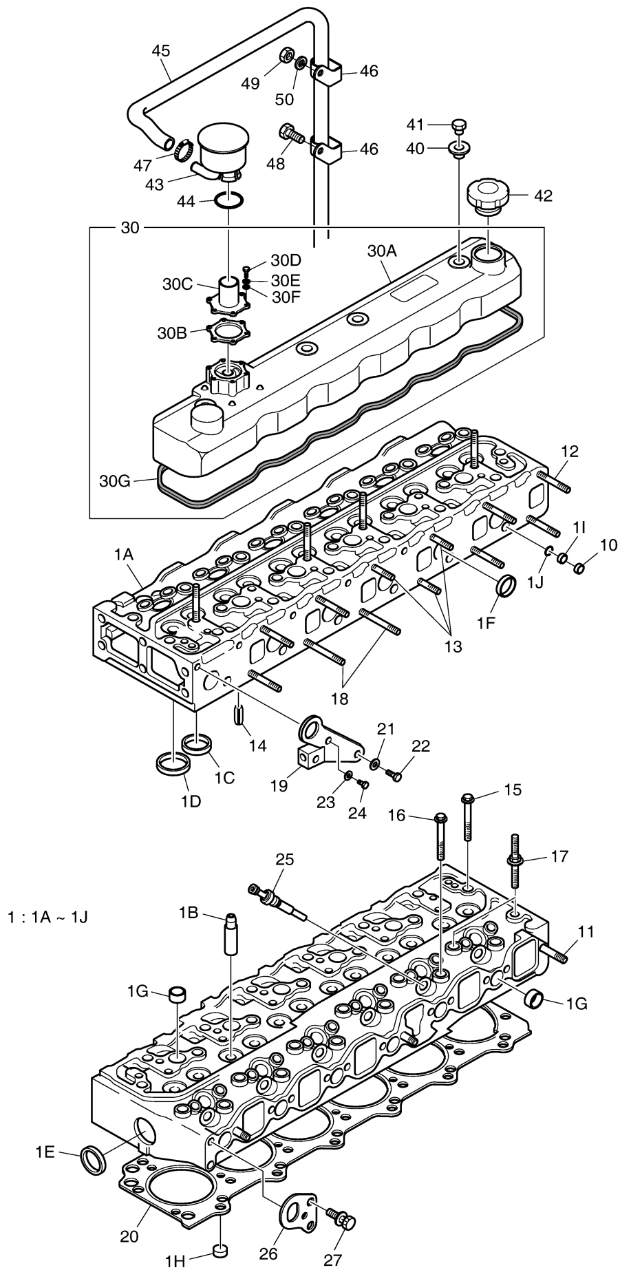
Fig. 005 CYLINDER HEAD
