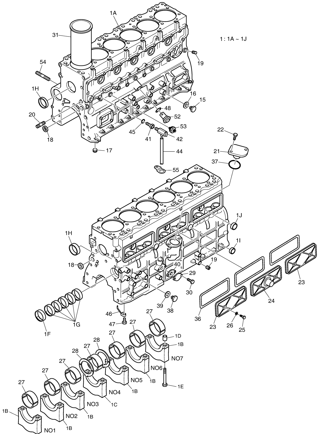
Fig. 001 CYLINDER BLOCK
