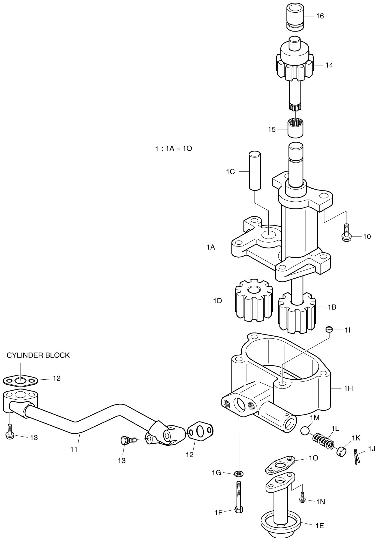
Fig. 007 OIL PUMP
