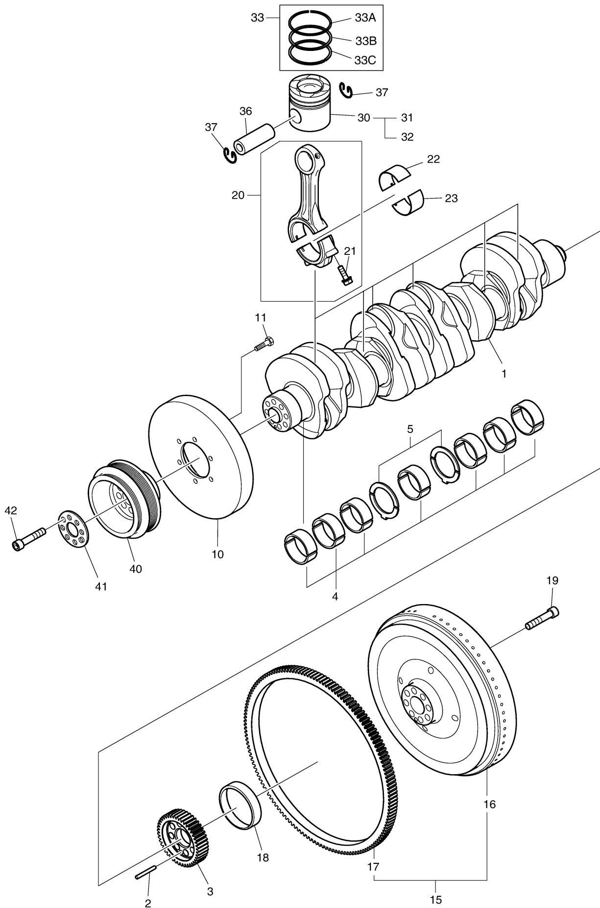
Fig. 016 DRIVING SYSTEM
