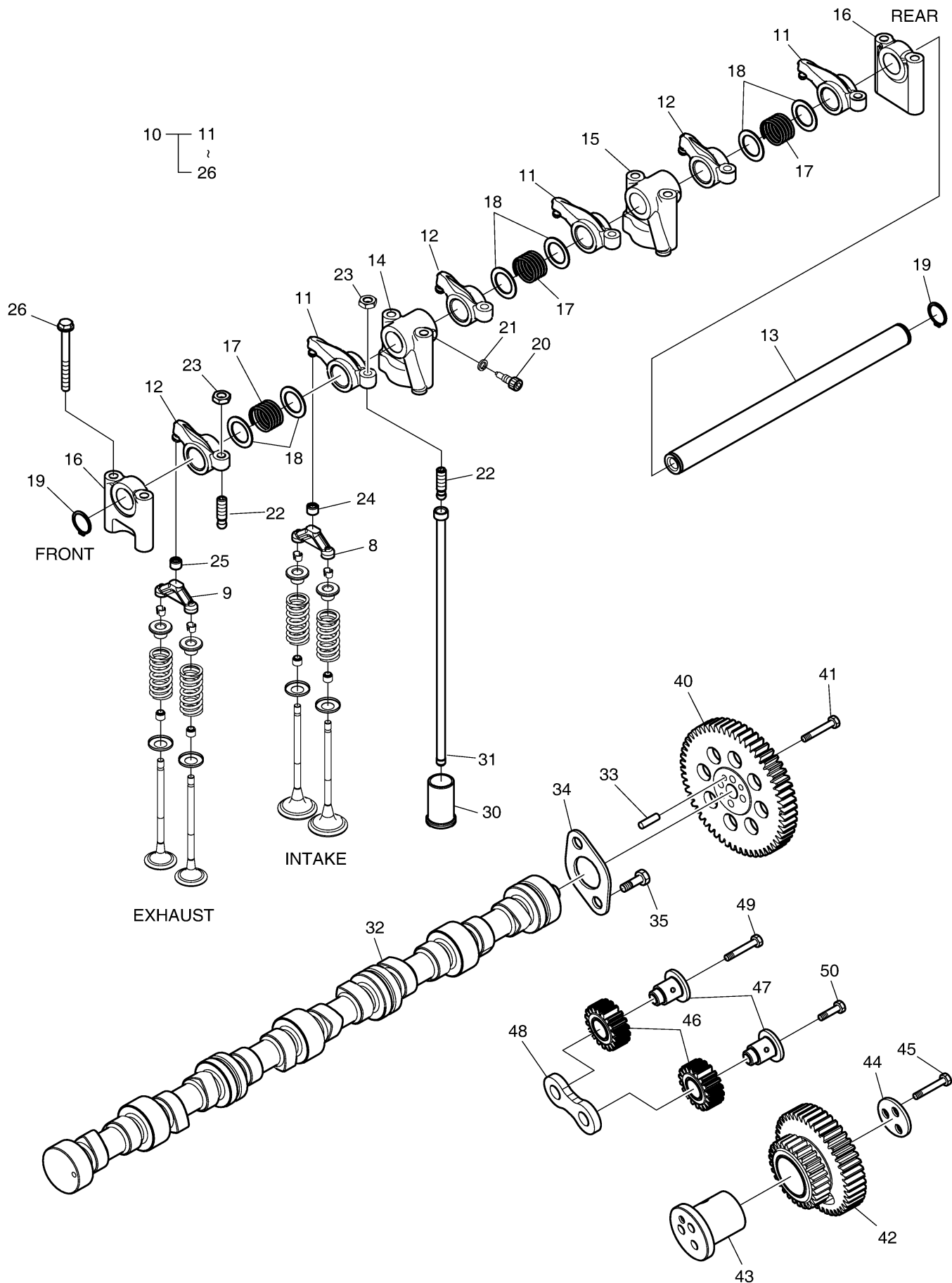
Fig. 019 TIMING SYSTEM
