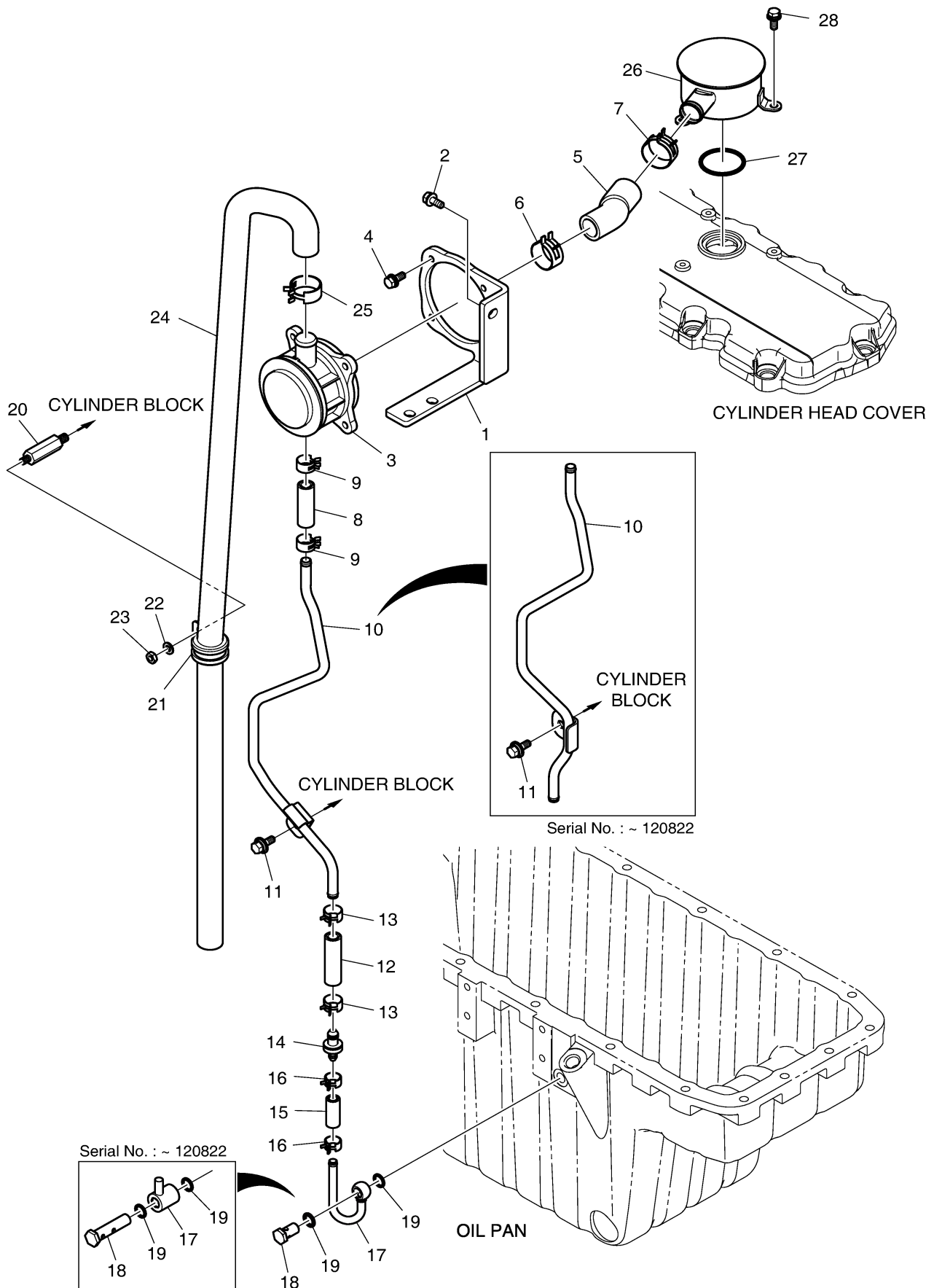
Fig. 006 BREATHER SYSTEM
