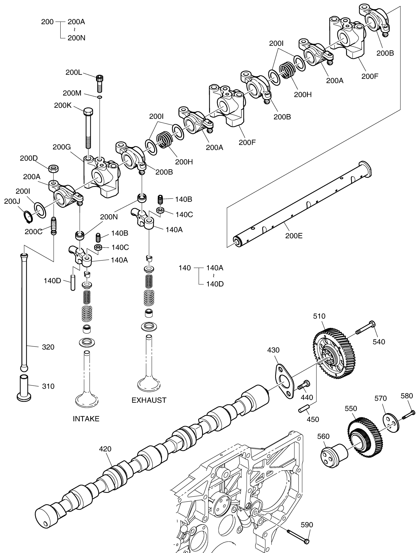
Fig. 009 TIMING SYSTEM
