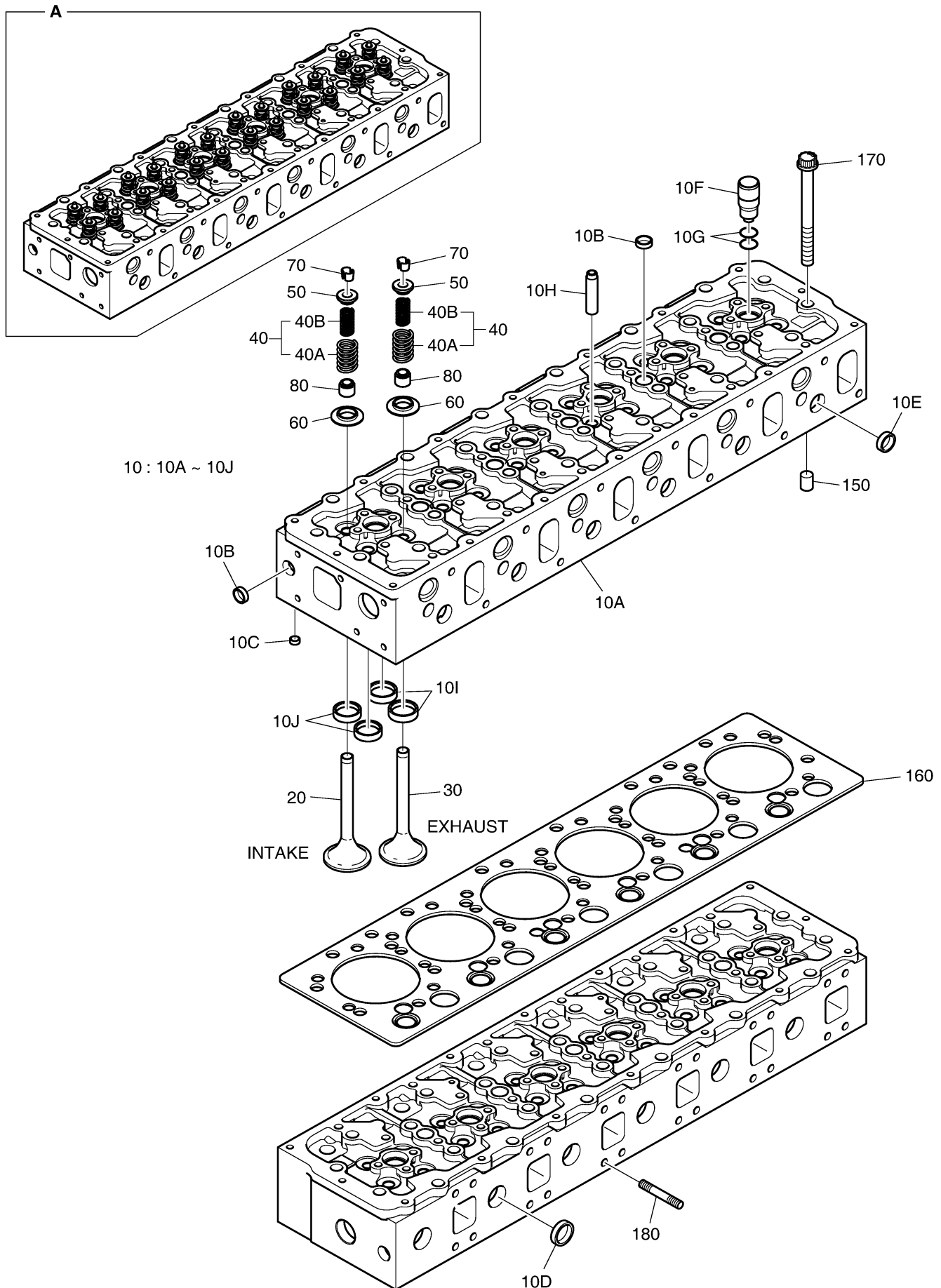
Fig. 007 CYLINDER HEAD
