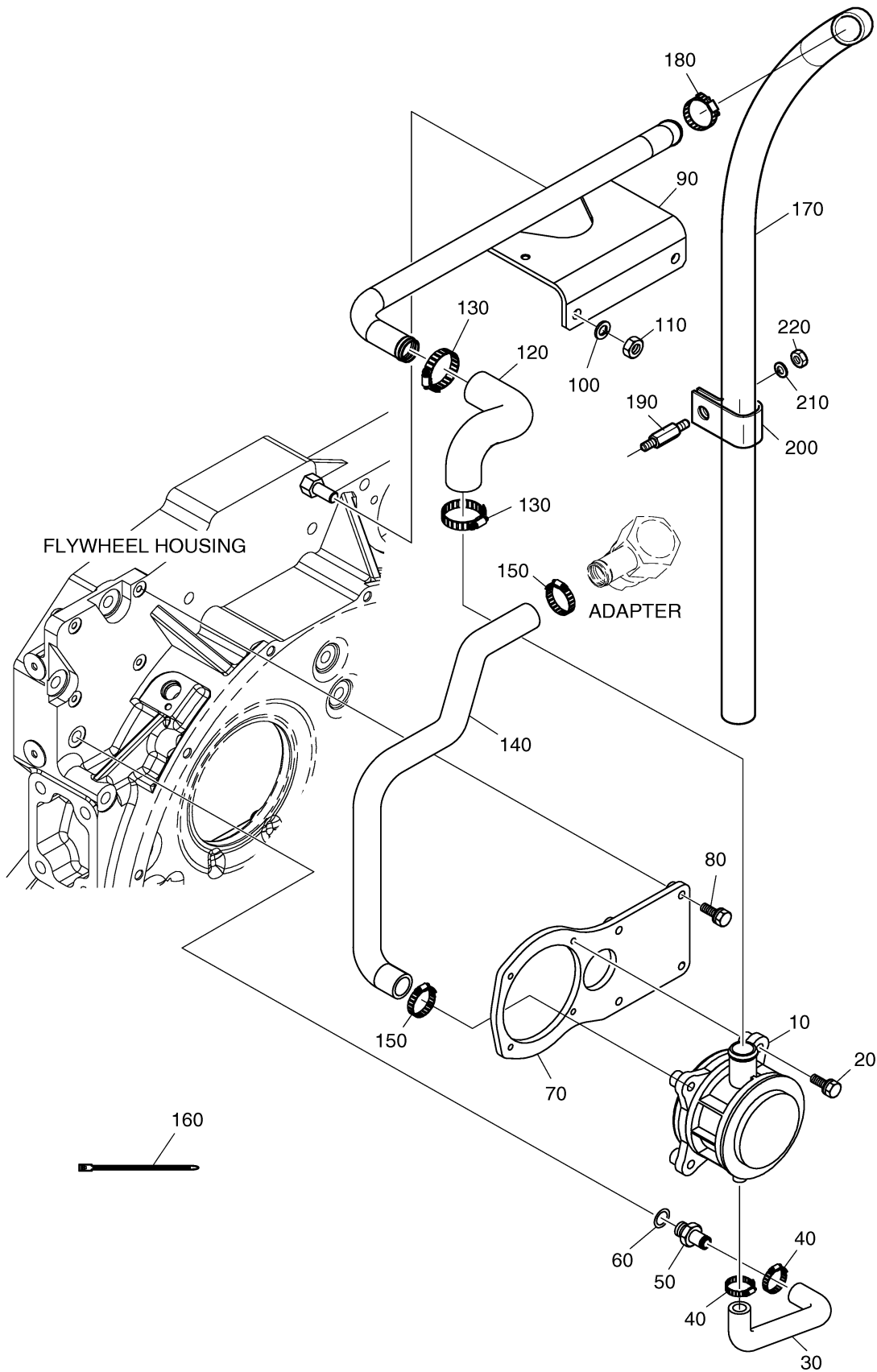
Fig. 005 BREATHER PIPE
