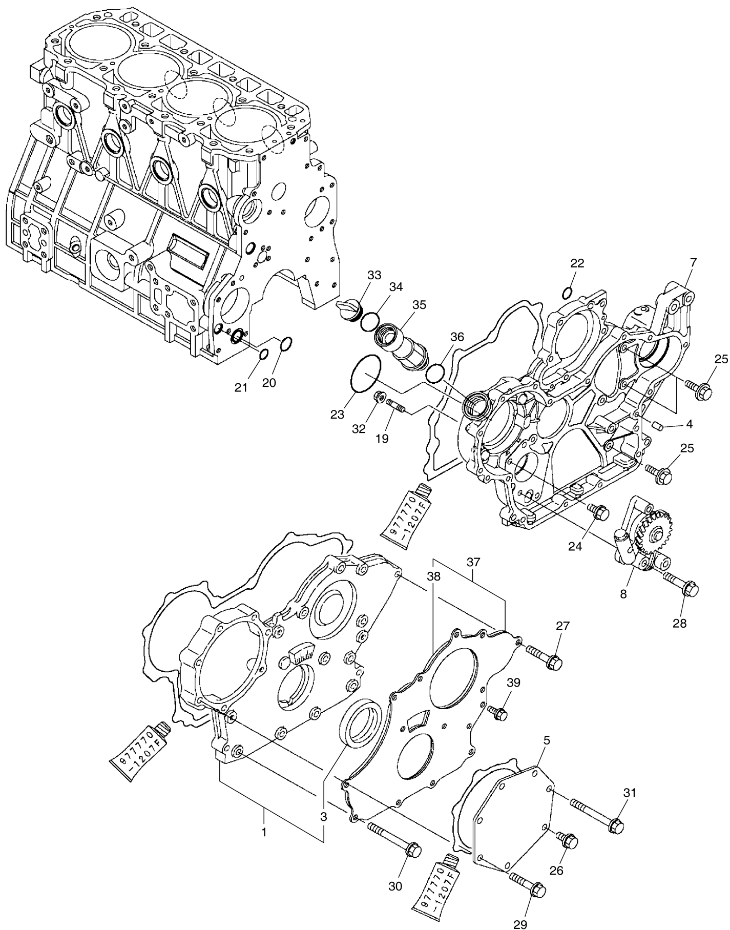
Fig. 012 GEAR HOUSING
