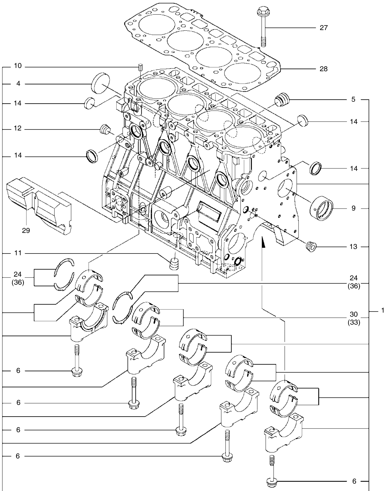
Fig. 011 CYLINDER BLOCK
