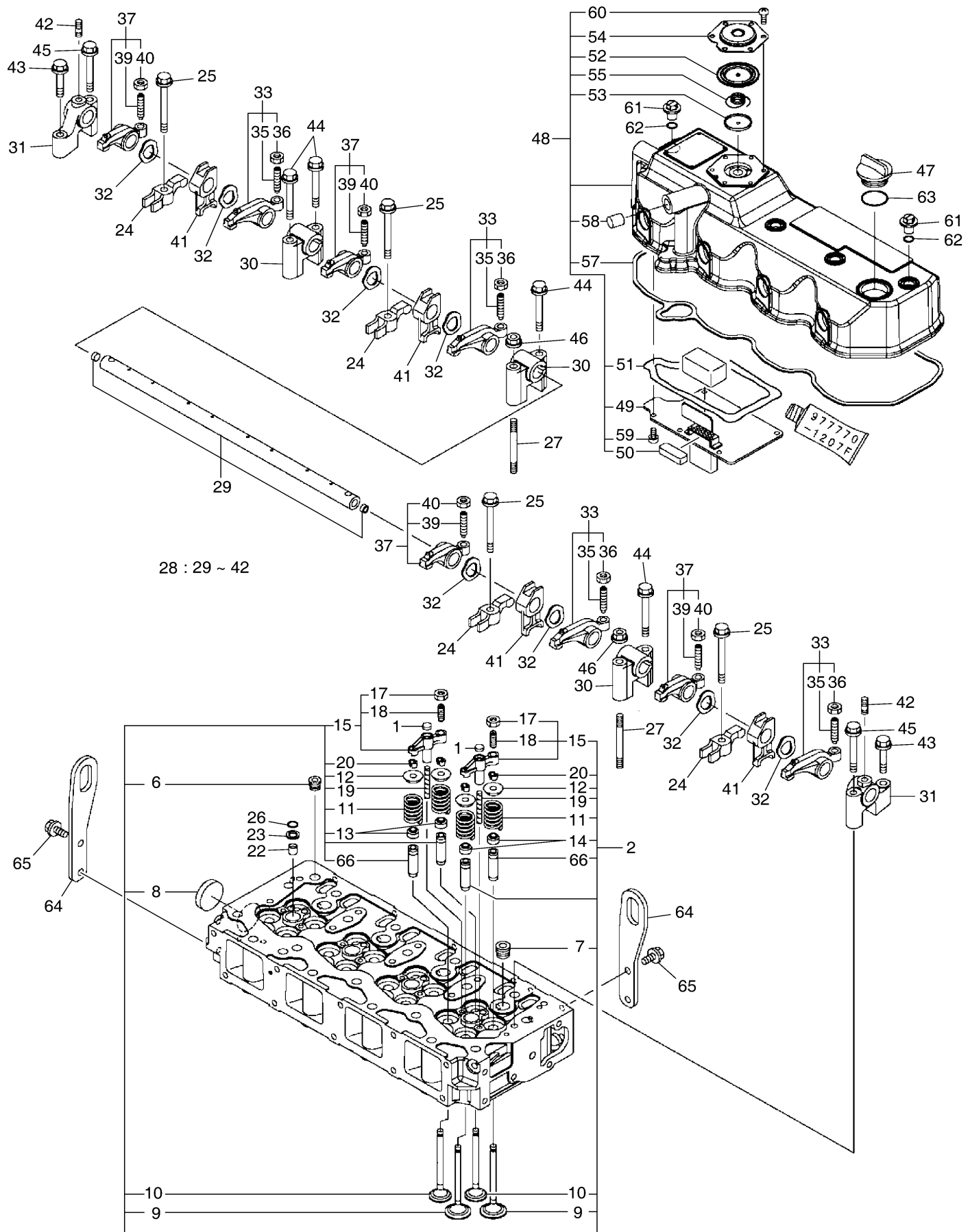
Fig. 014 CYLINDER HEAD & BONNET
