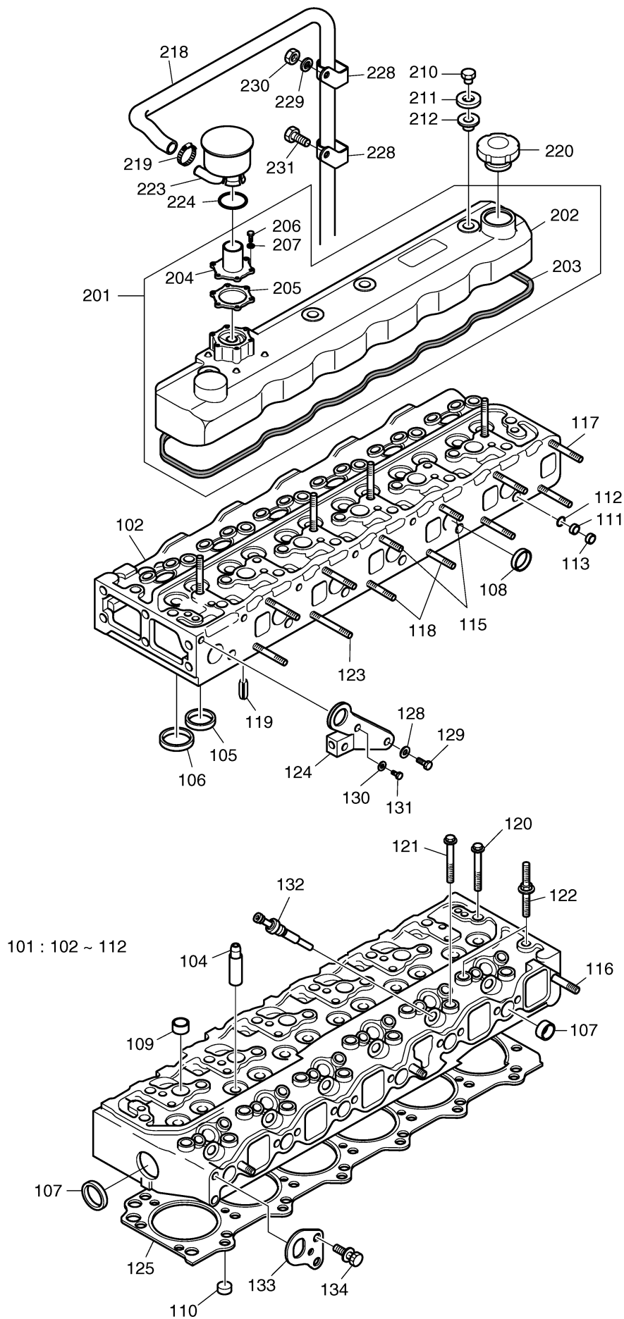
Fig. 005 CYLINDER HEAD
