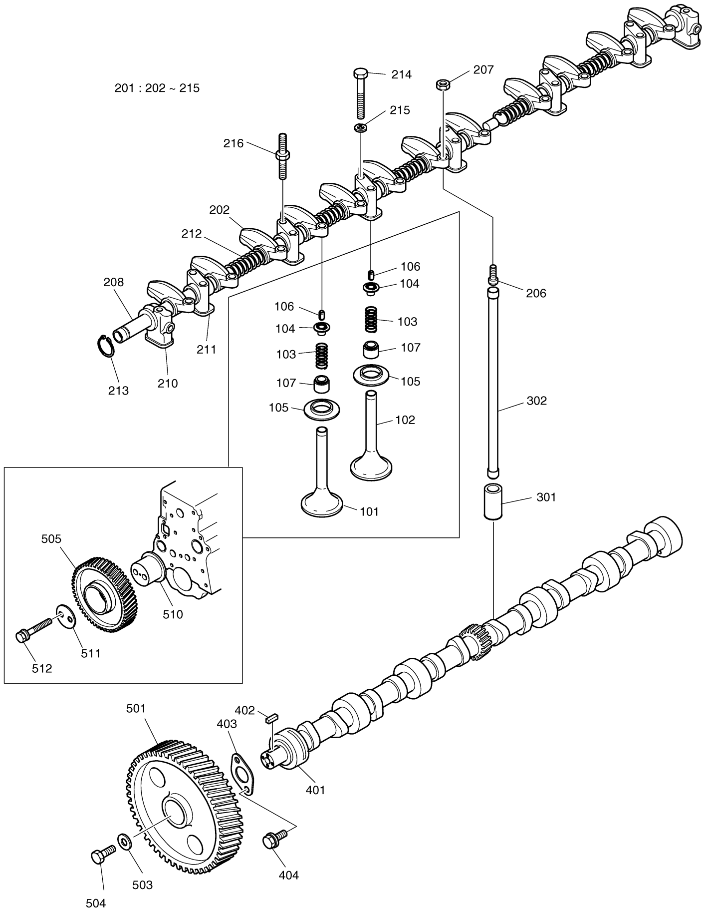
Fig. 006 VALVE MECHANISM
