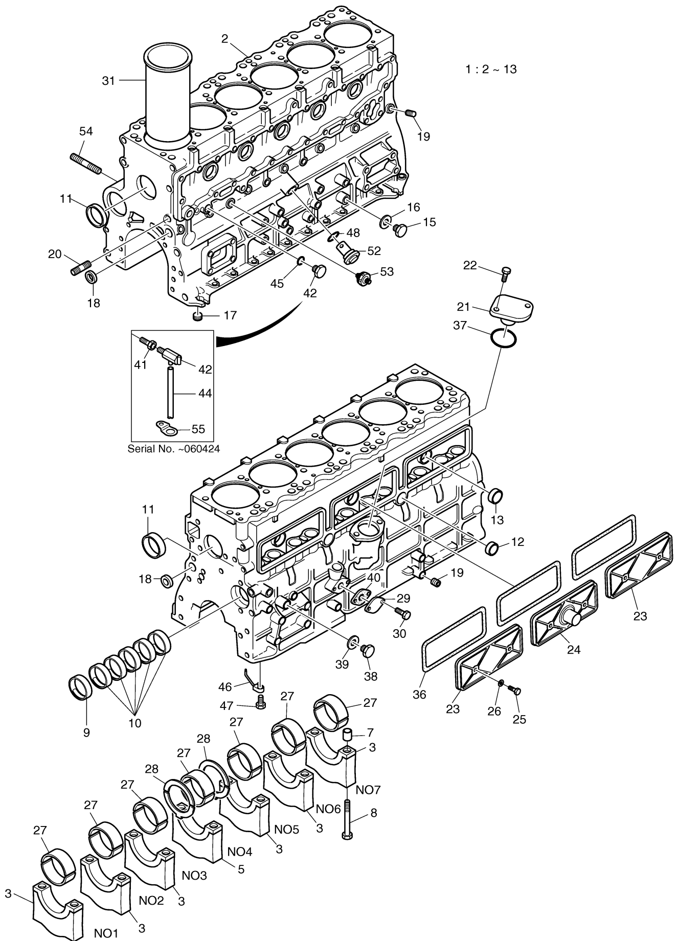
Fig. 001 CYLINDER BLOCK
