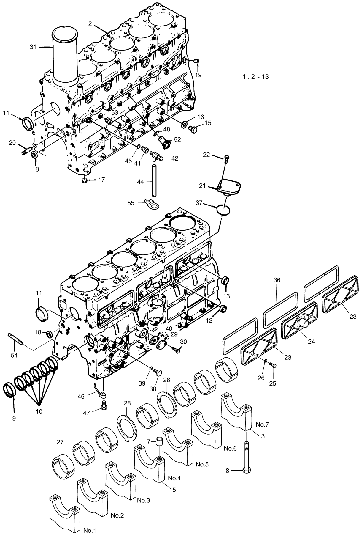
Fig. 001 CYLINDER BLOCK
