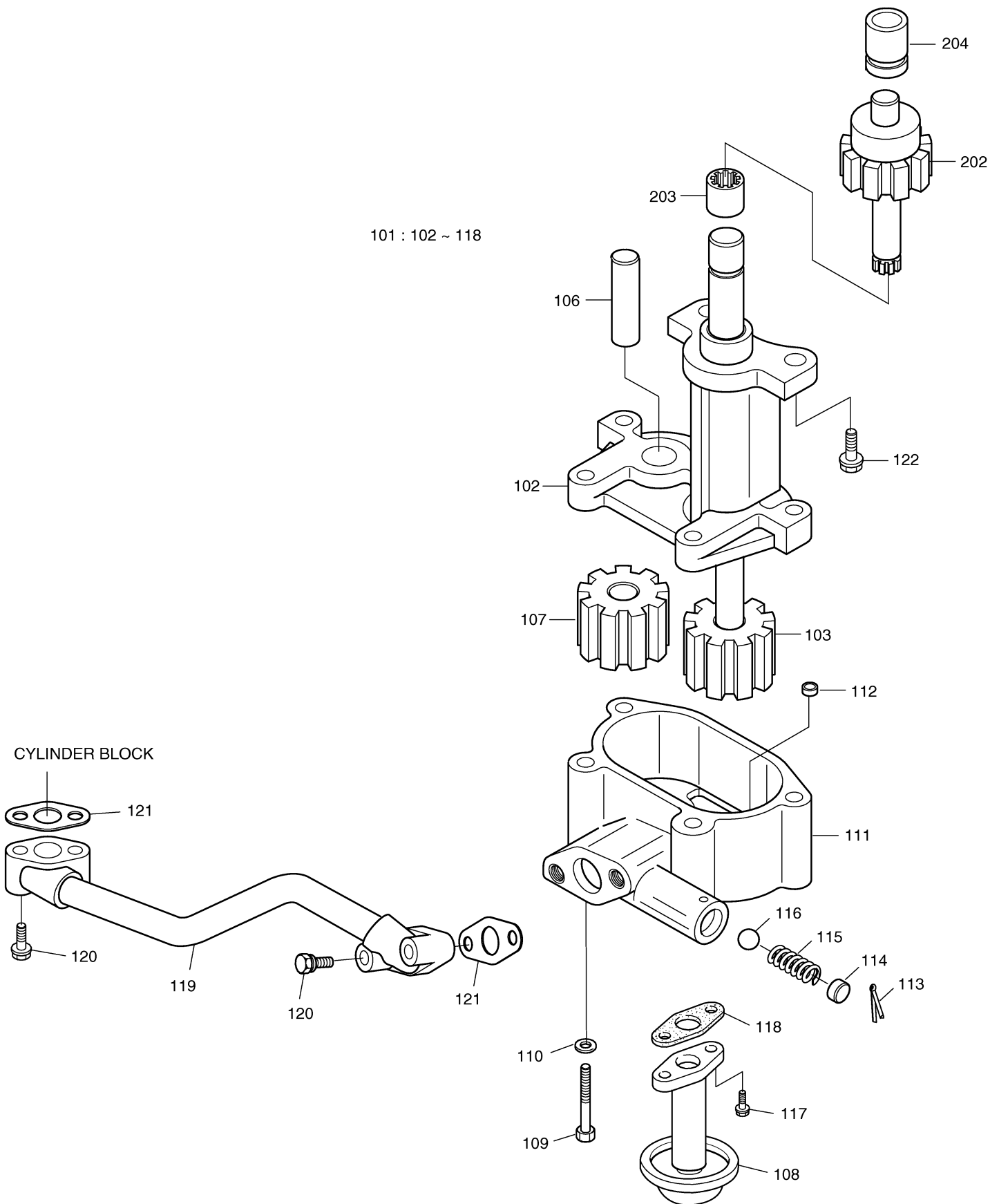
Fig. 007 OIL PUMP
