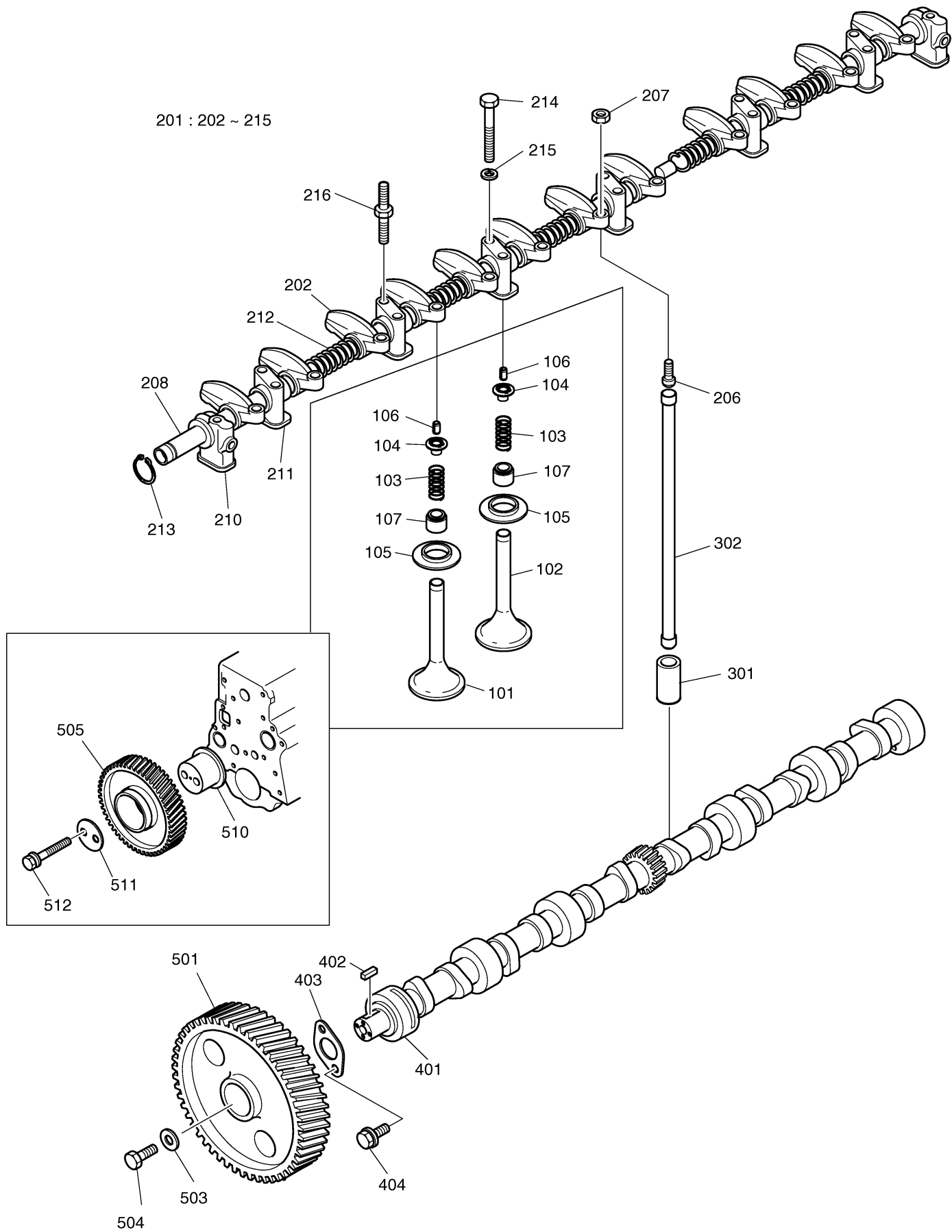
Fig. 006 VALVE MECHANISM
