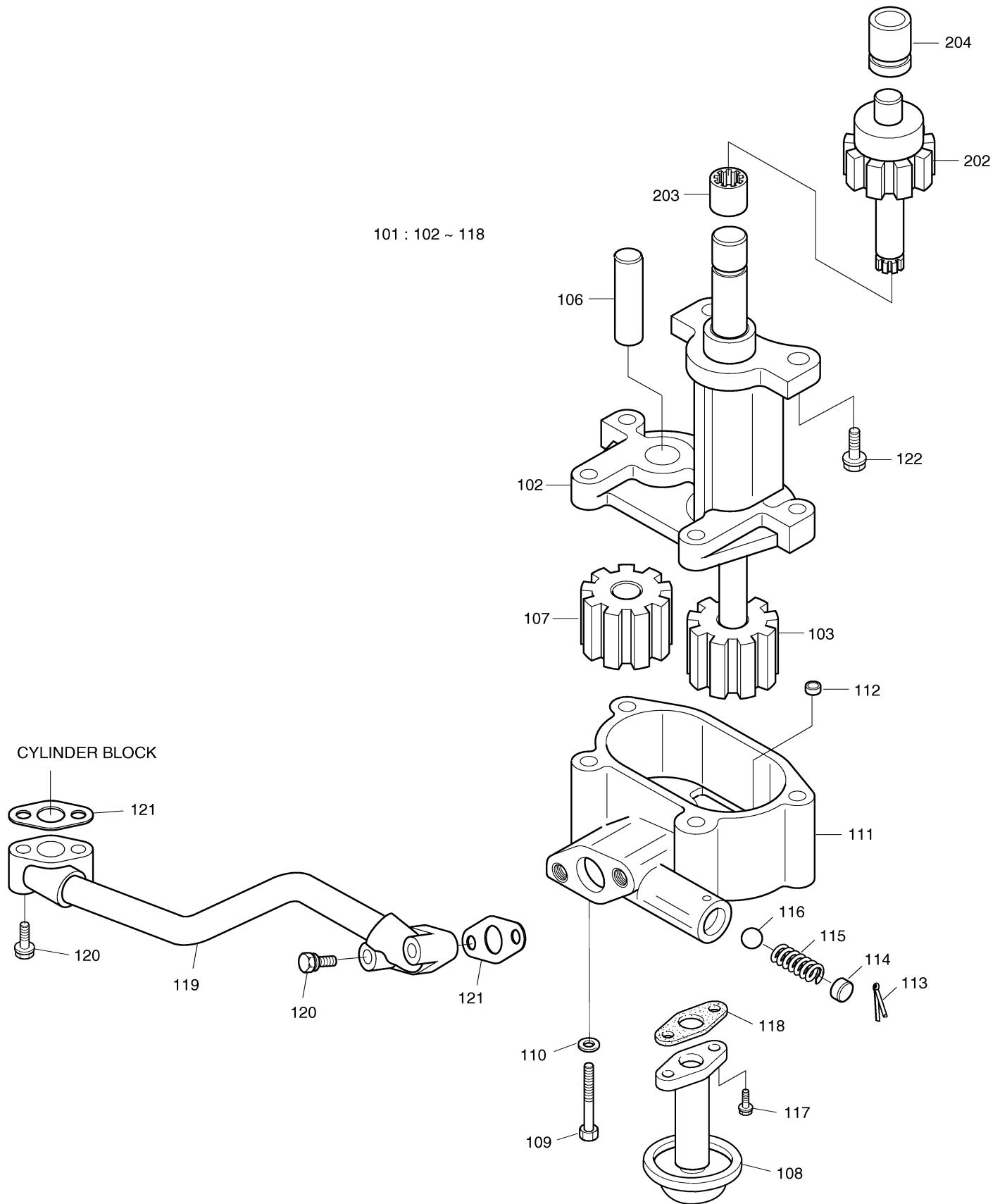
Fig. 007 OIL PUMP
