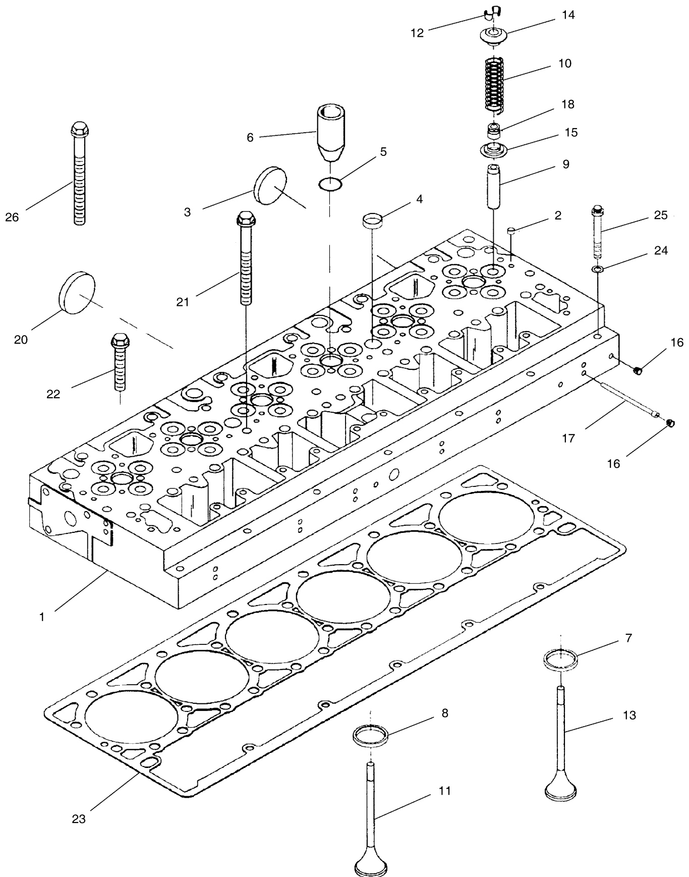
Fig. 059 CYLINDER HEAD
