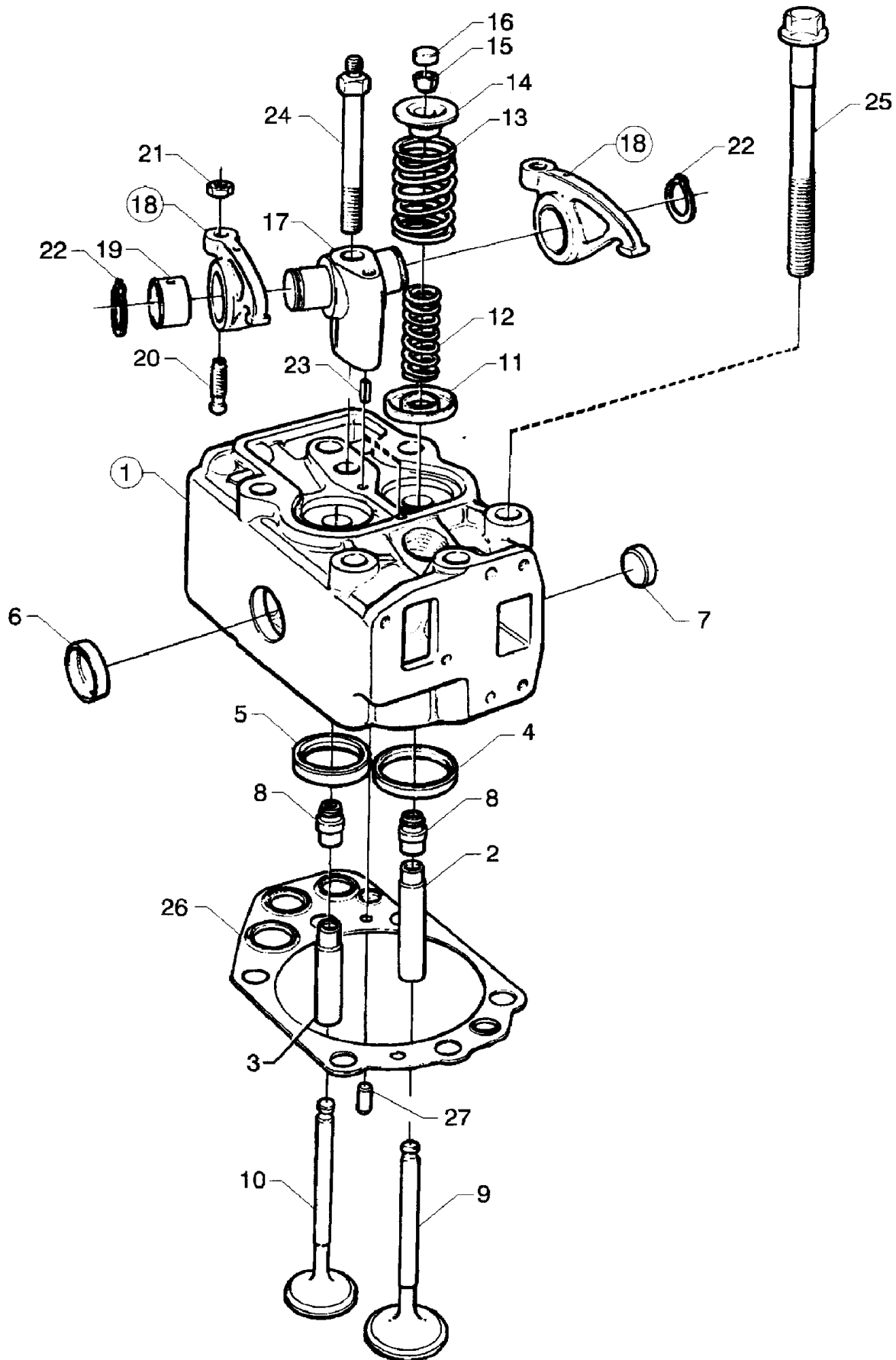
Fig. G010-6 CYLINDER HEAD
