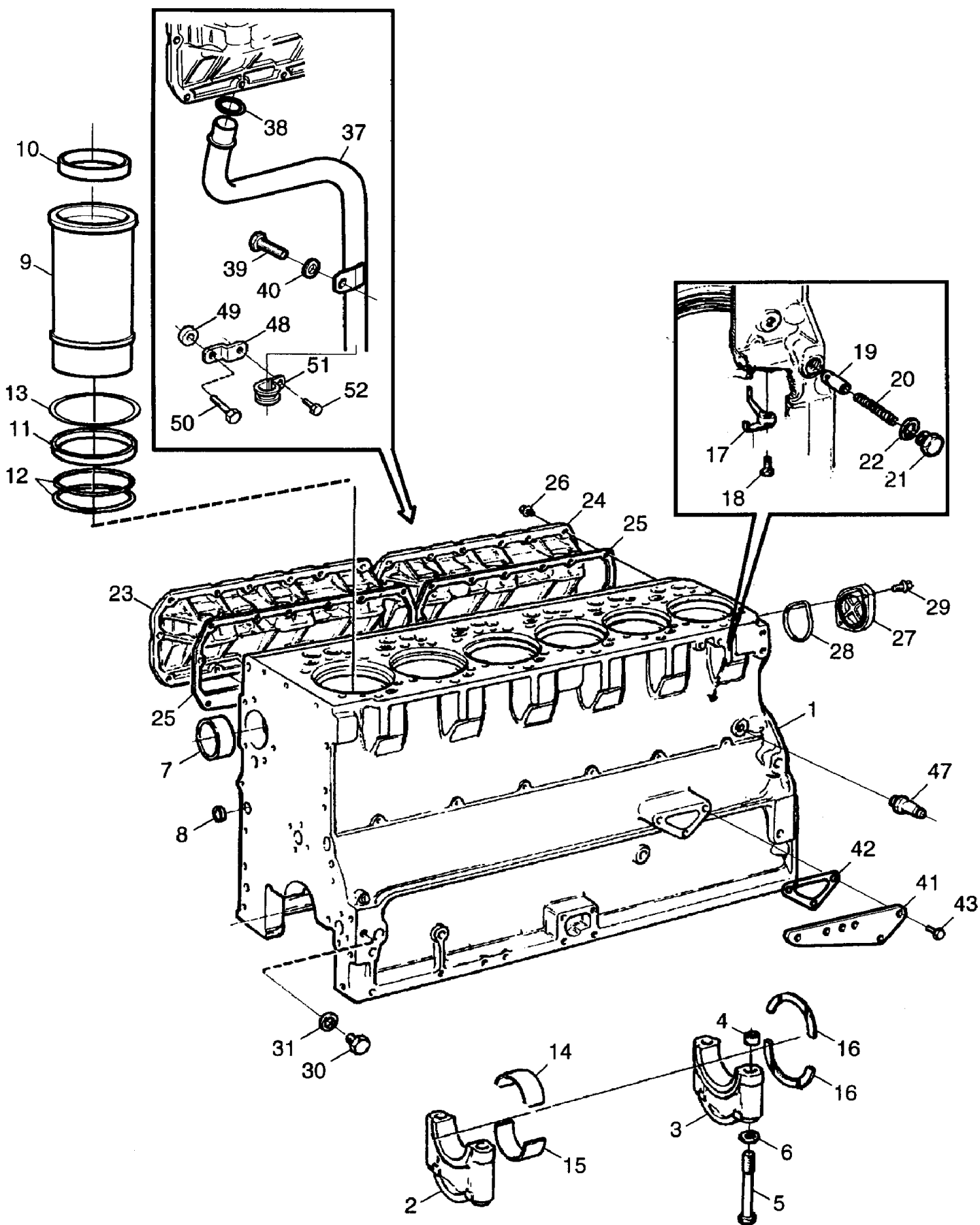
Fig. G010-10 CYLINDER BLOCK
