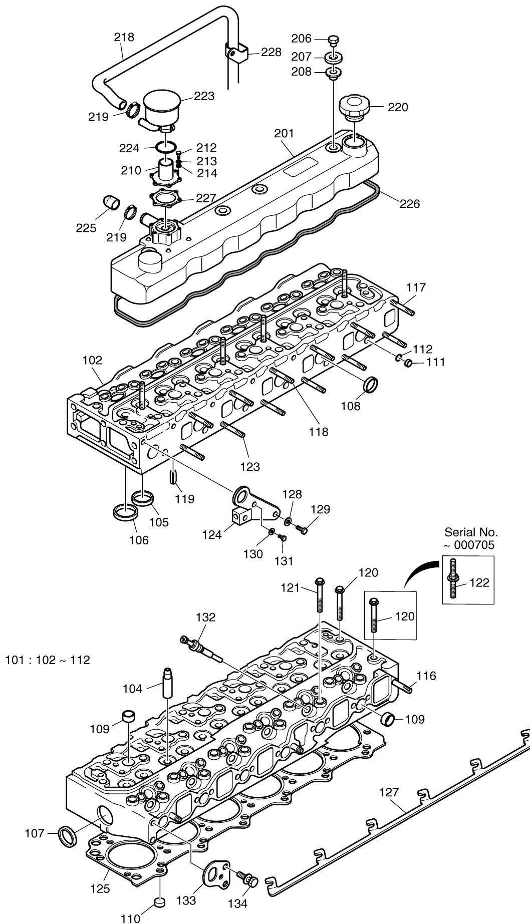
Fig. 005 CYLINDER HEAD
