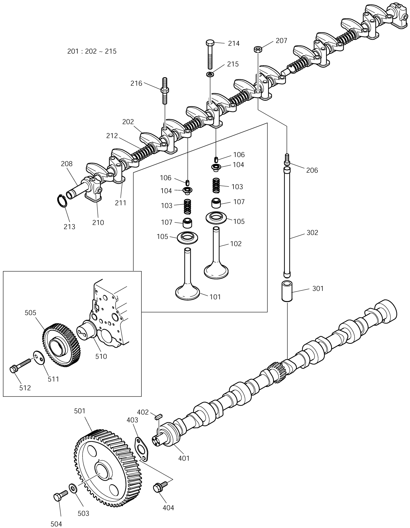
Fig. 006 VALVE MECHANISM
