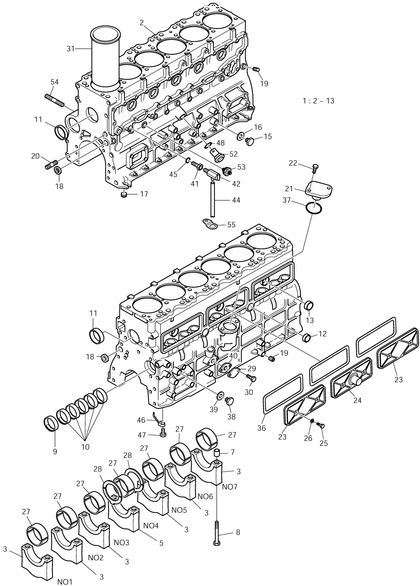
Fig. 001 CYLINDER BLOCK
