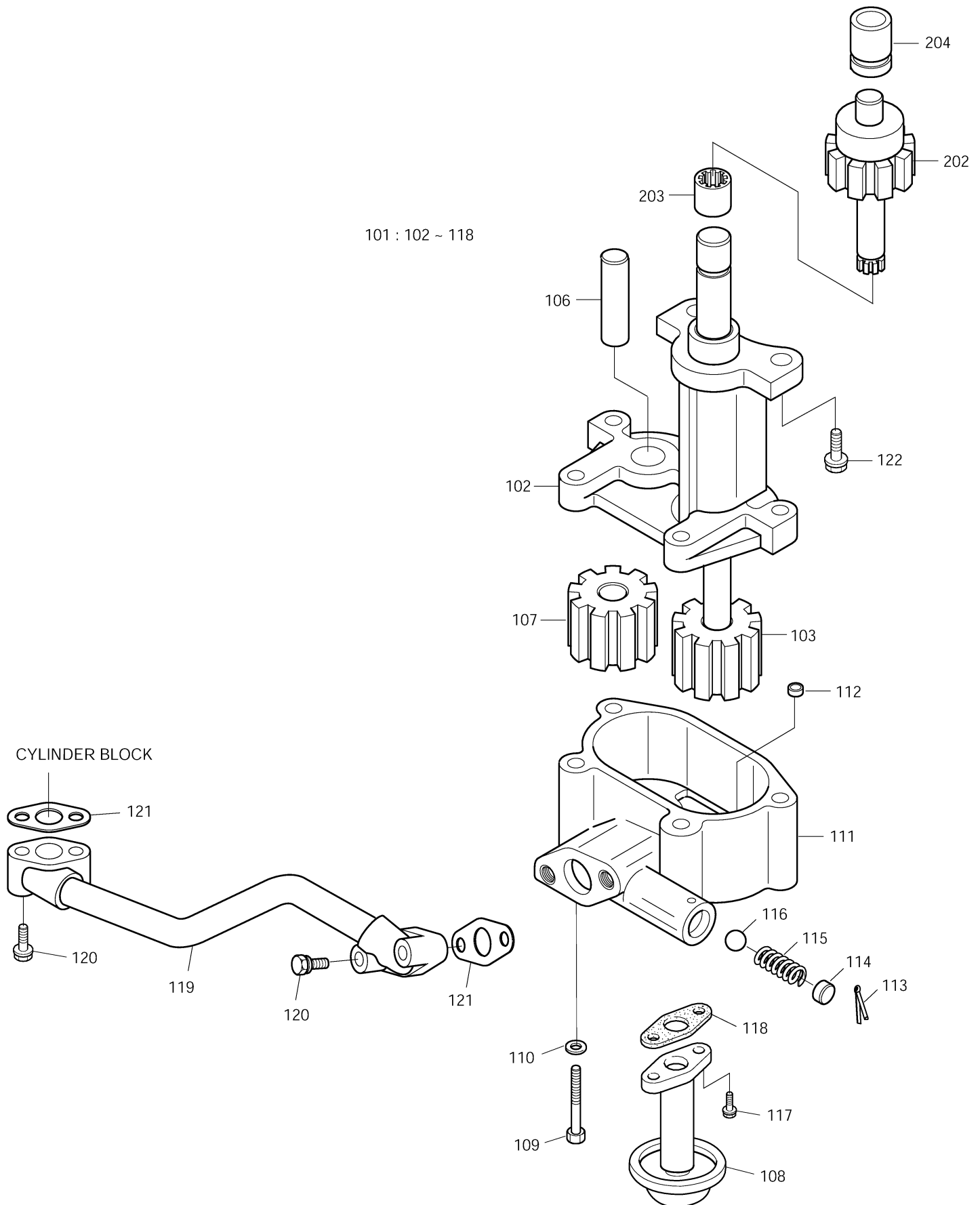
Fig. 007 OIL PUMP
