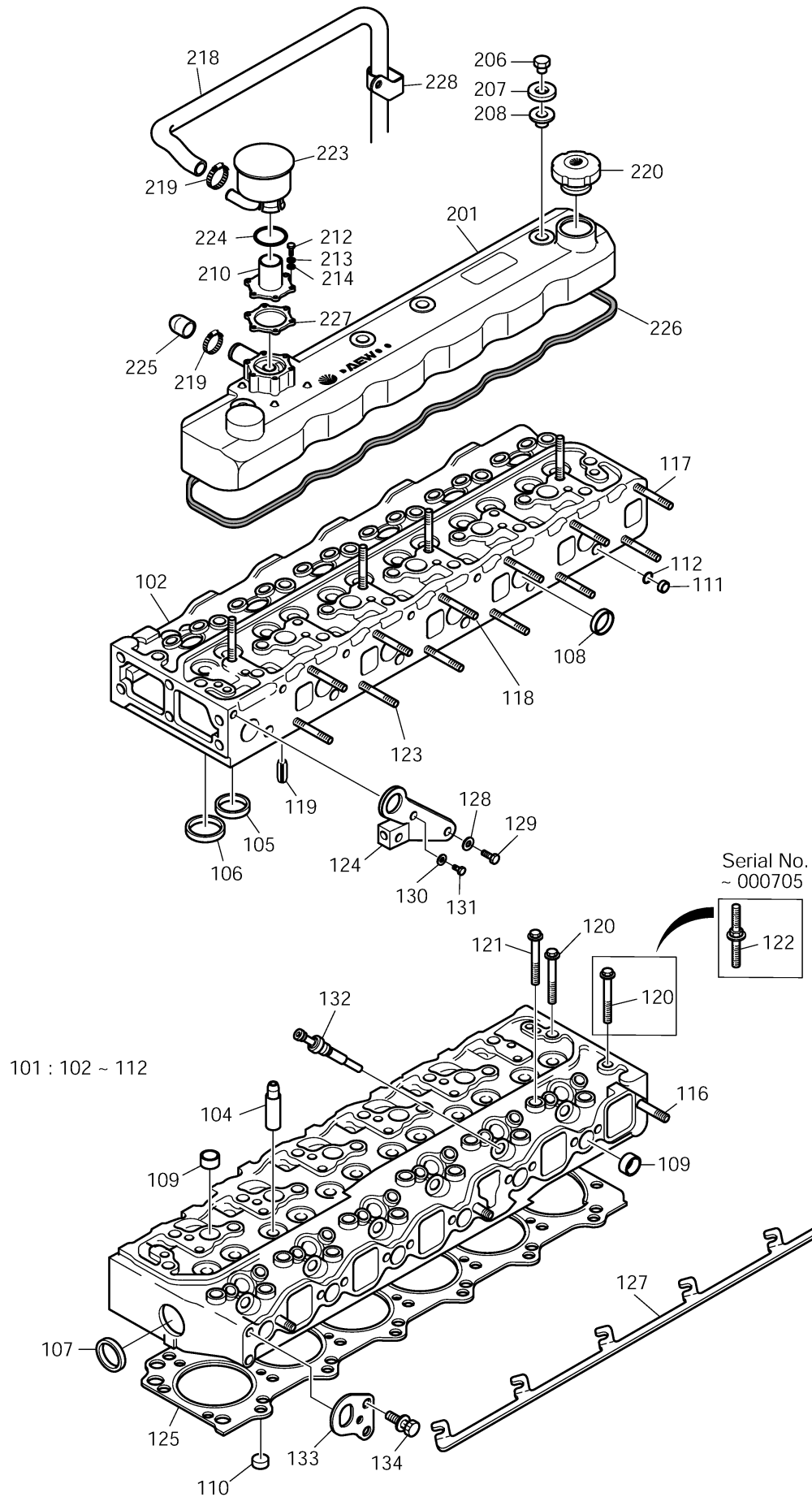
Fig. 005 CYLINDER HEAD
