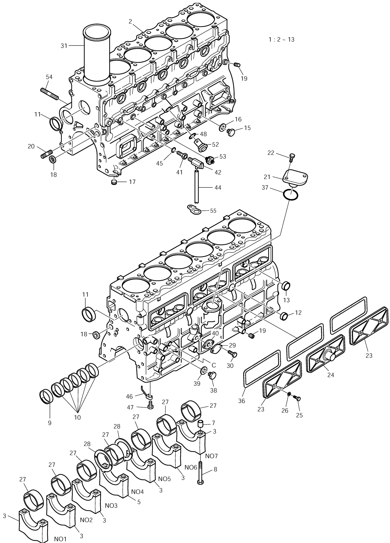
Fig. 001 CYLINDER BLOCK
