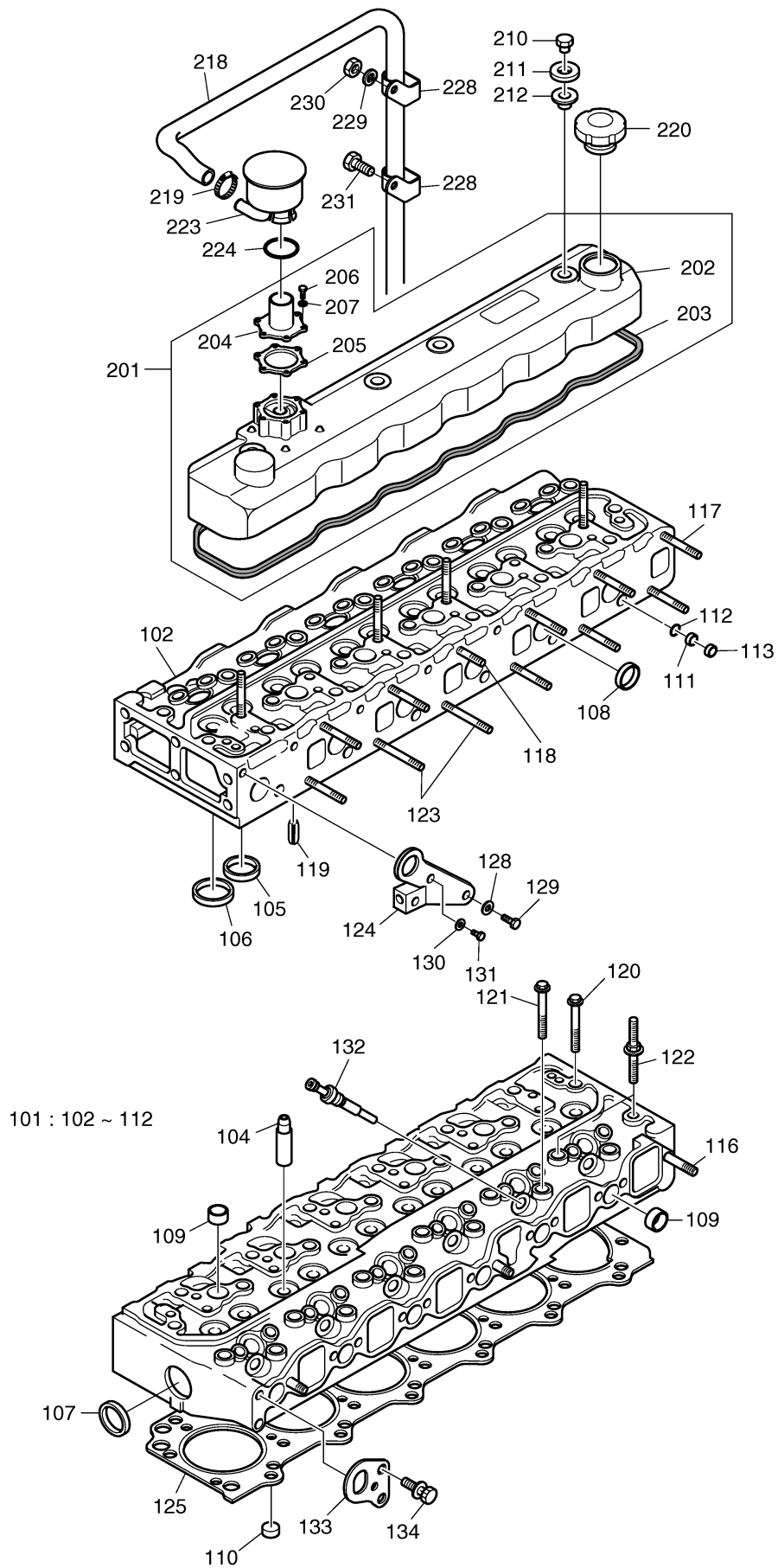
Fig. 005 CYLINDER HEAD
