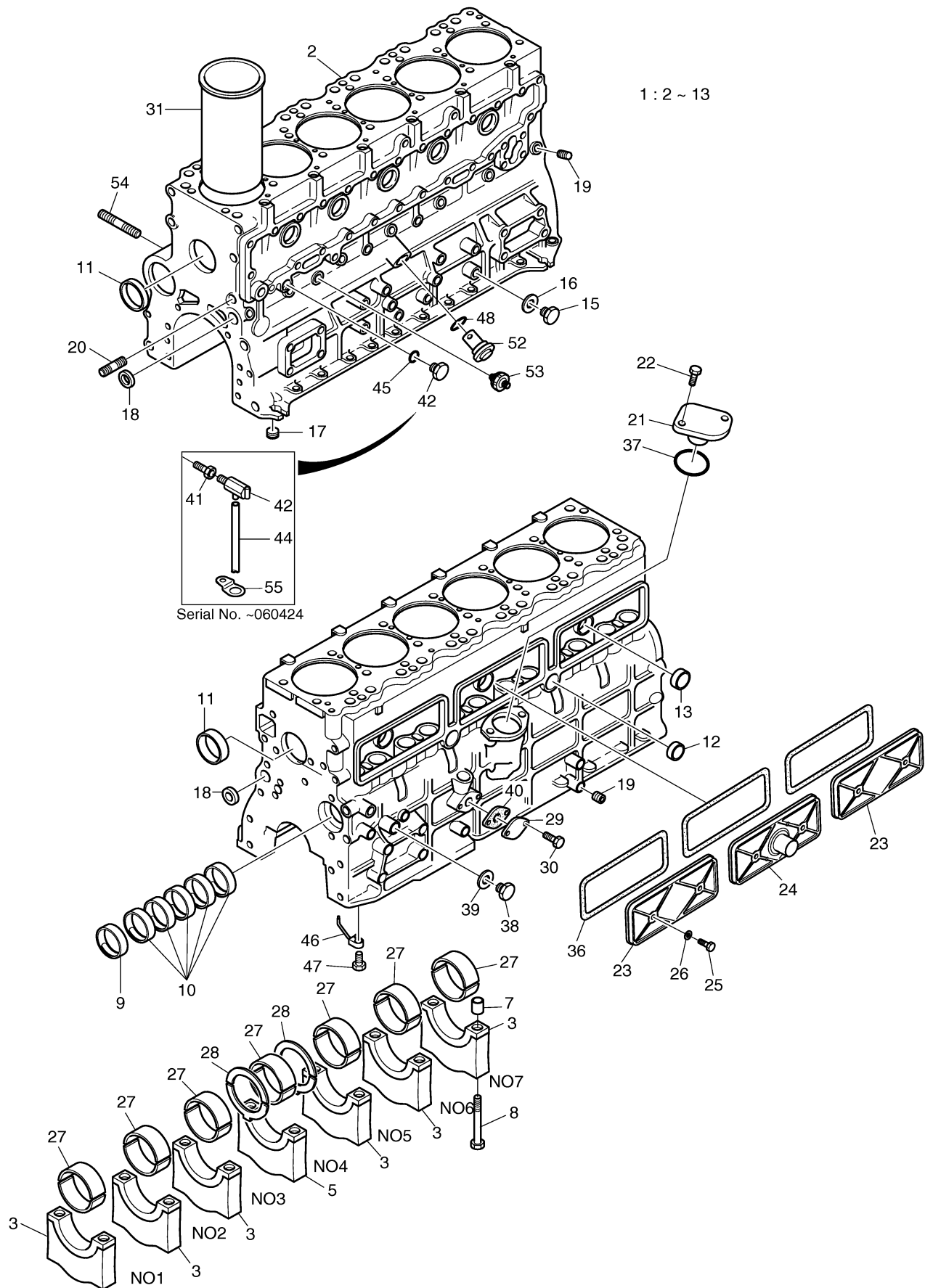
Fig. 001 CYLINDER BLOCK
