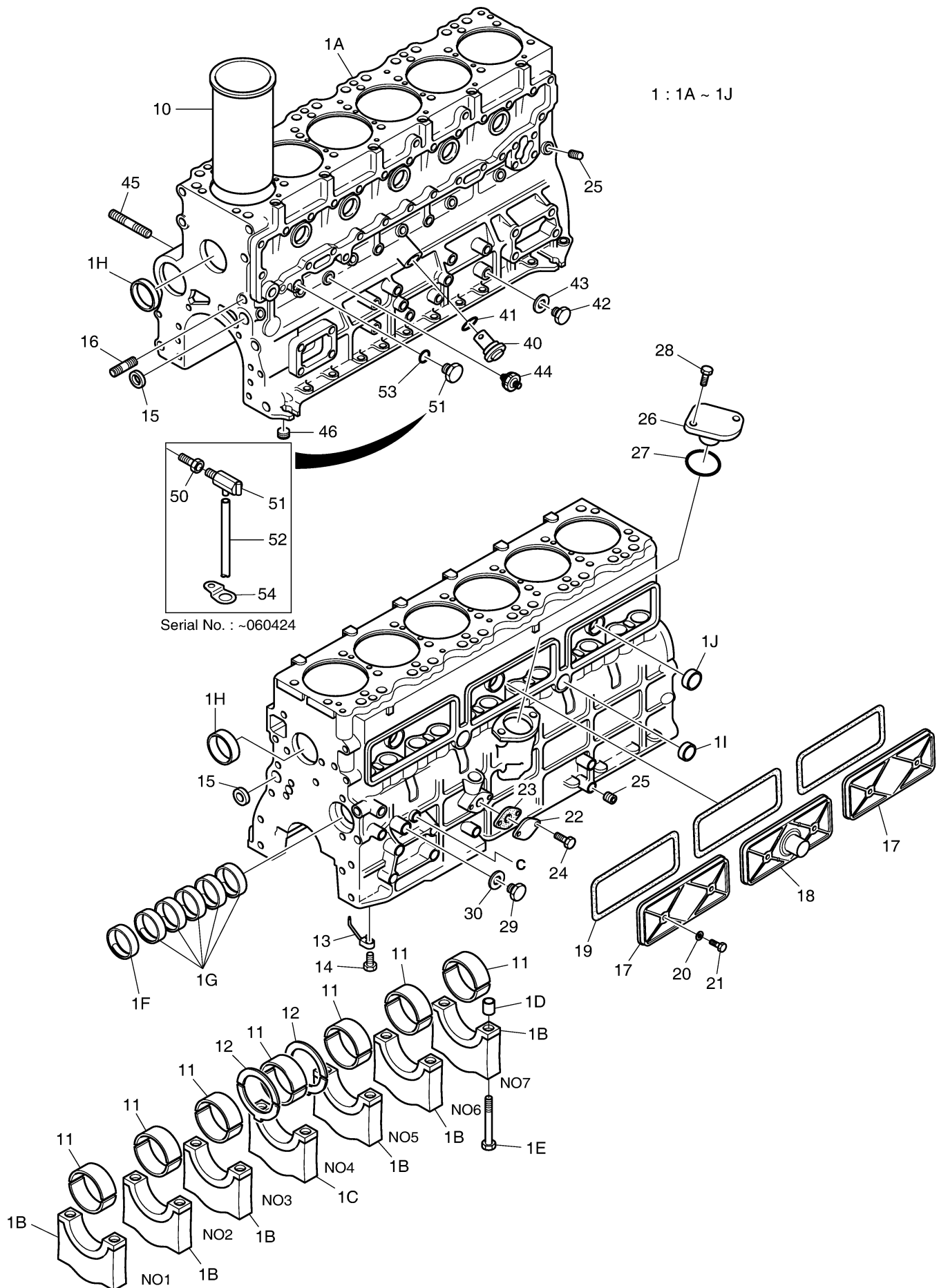
Fig. 001 CYLINDER BLOCK
