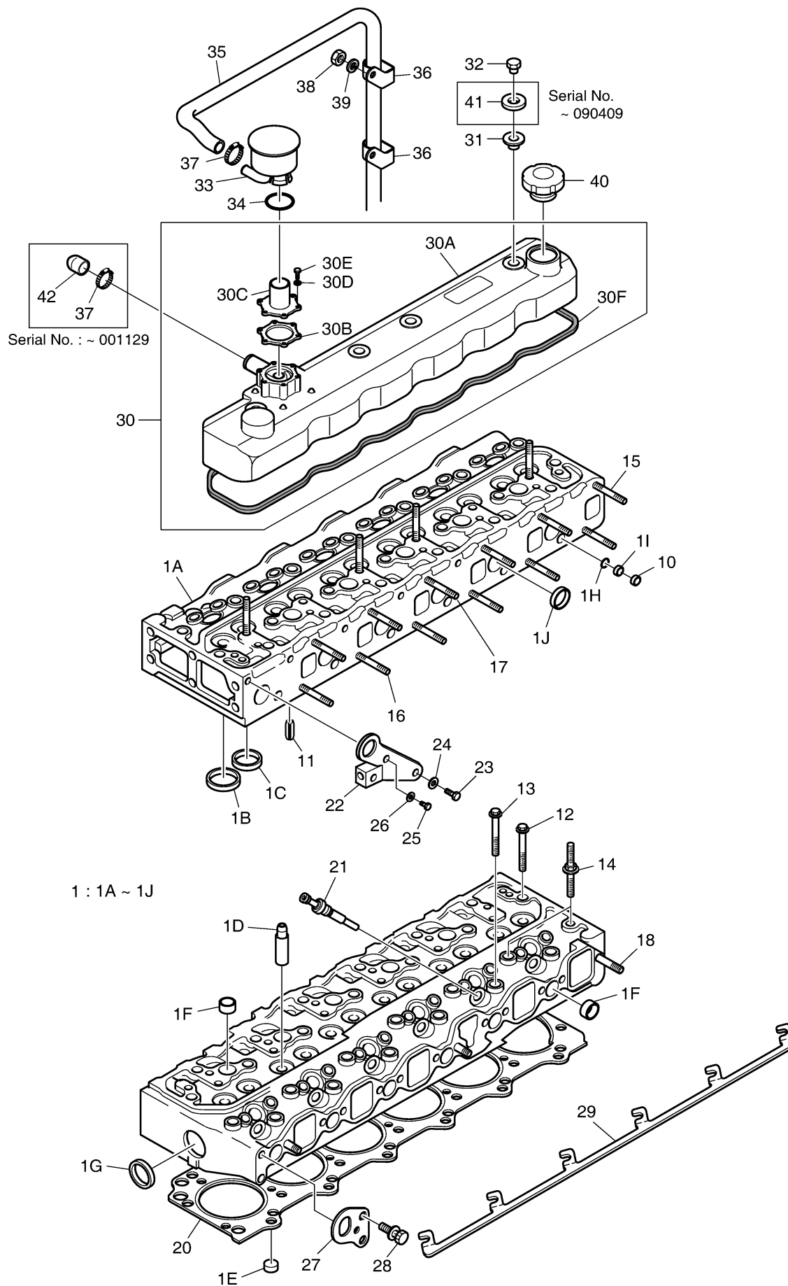
Fig. 005 CYLINDER HEAD
