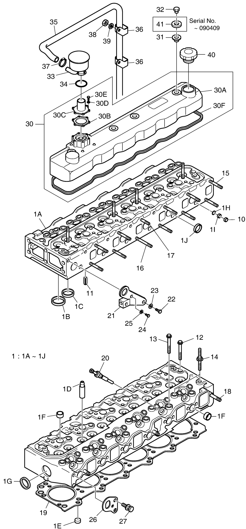
Fig. 005 CYLINDER HEAD
