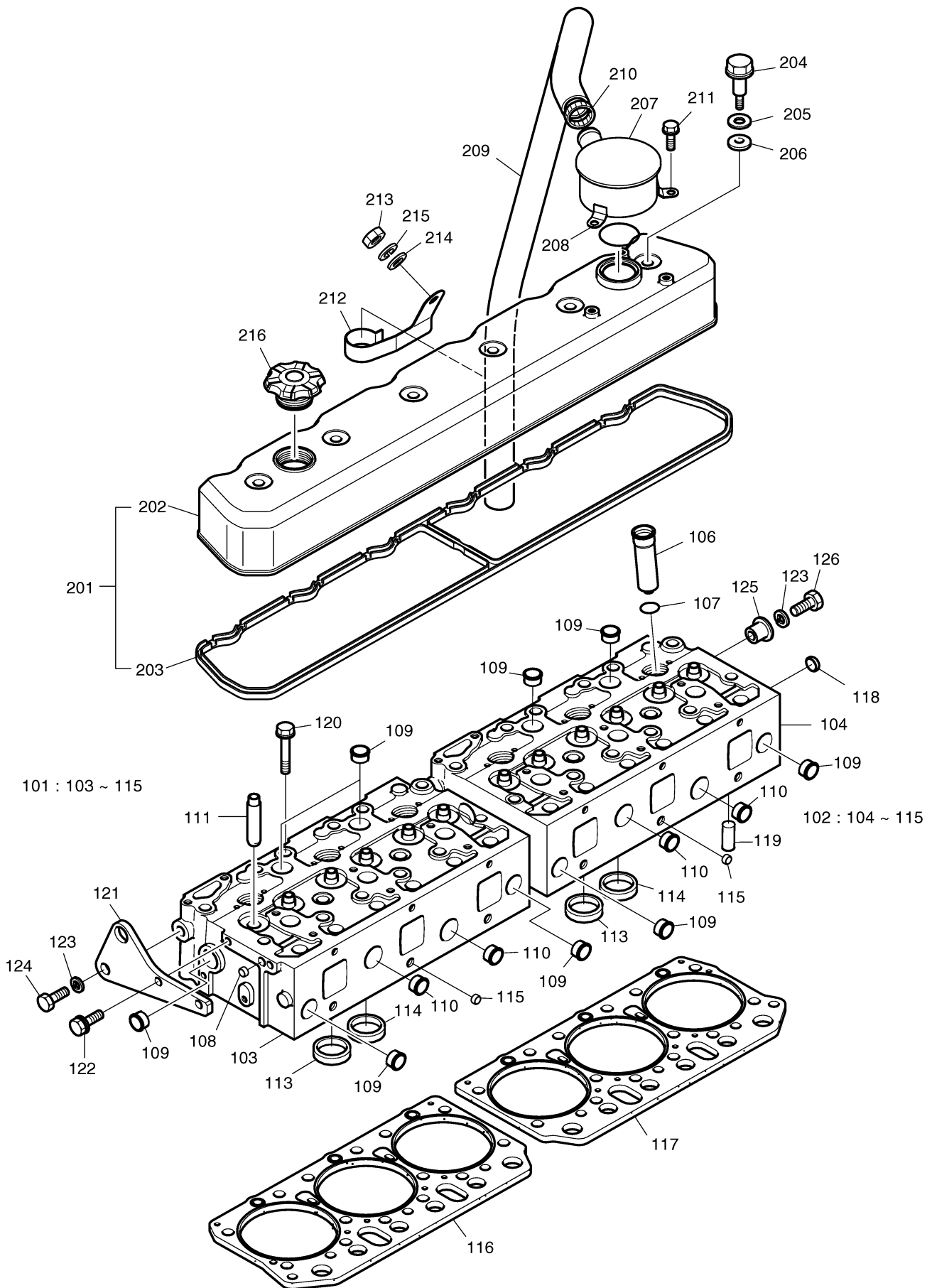
Fig. 017 CYLINDER HEAD
