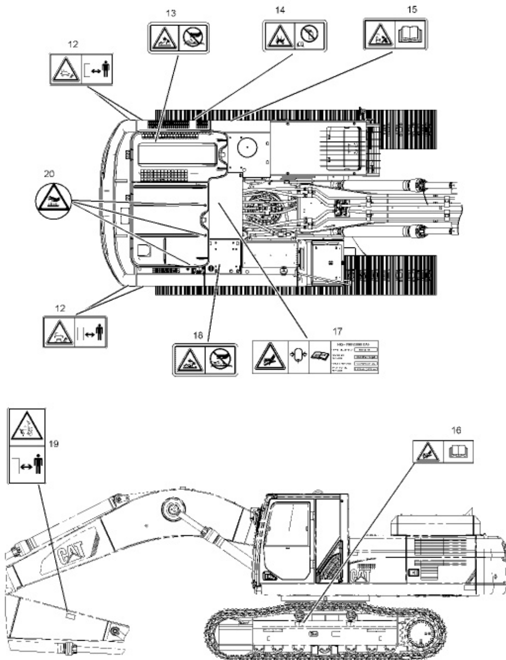
Illustration 2 Top and side view of machine
