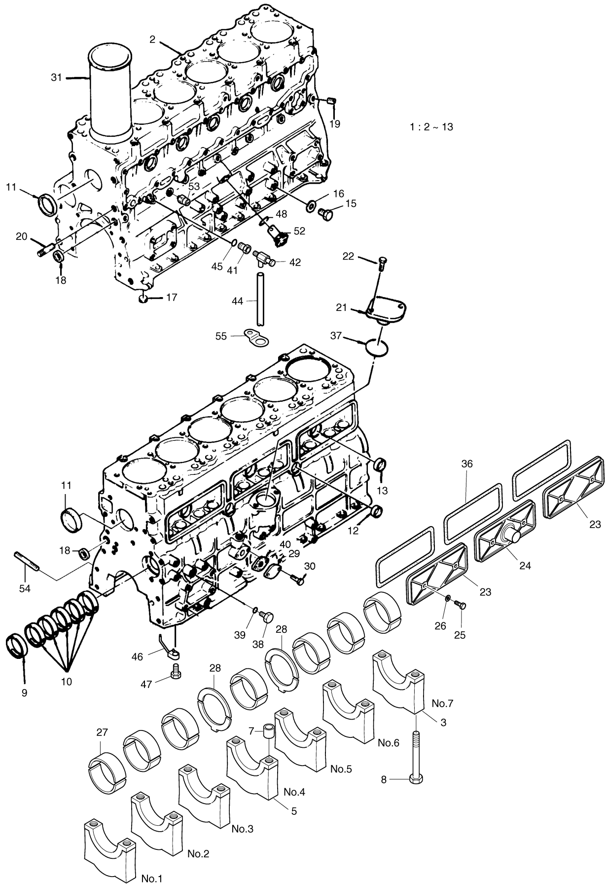
Fig. 001 CYLINDER BLOCK
