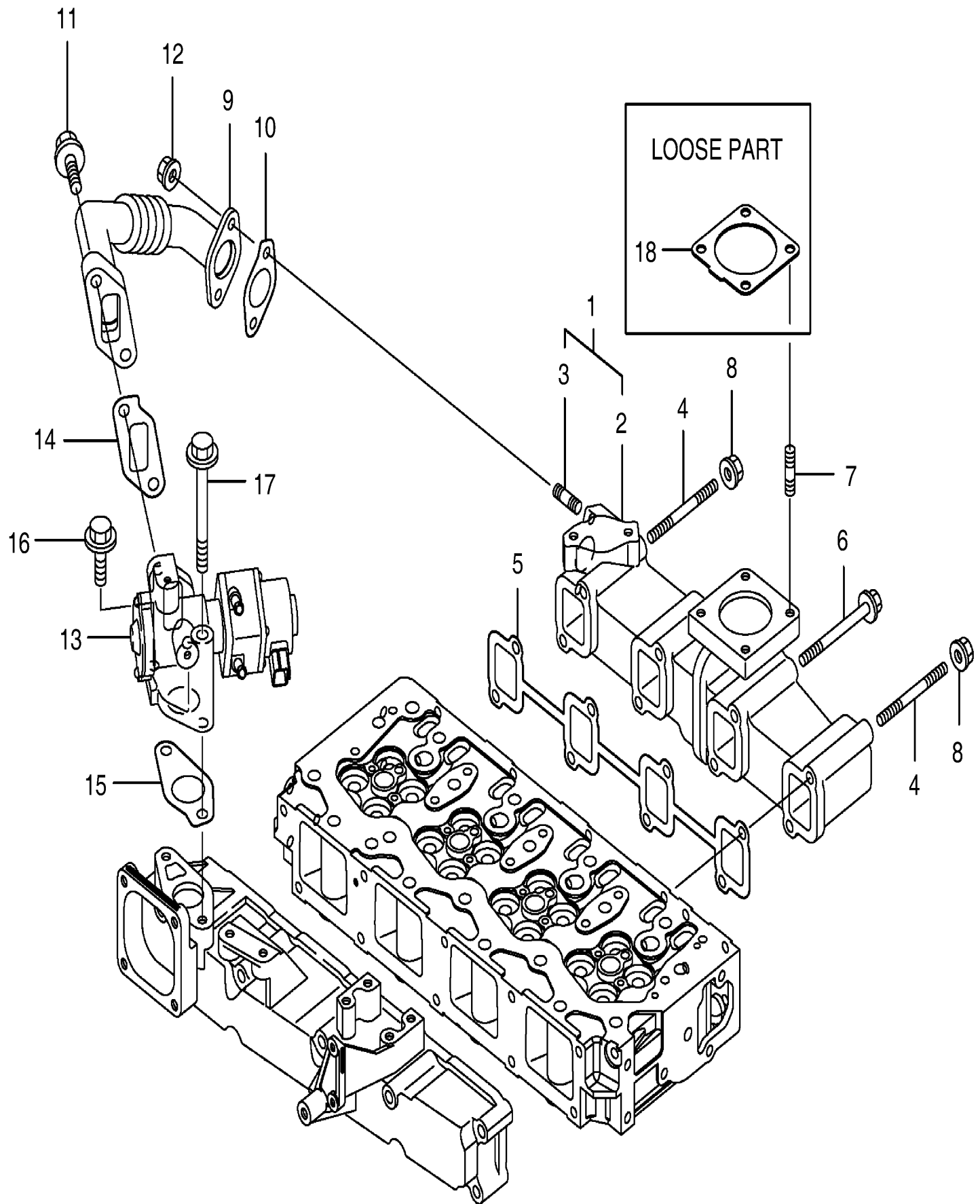
Fig. 016 EXHAUST MANIFOLD
