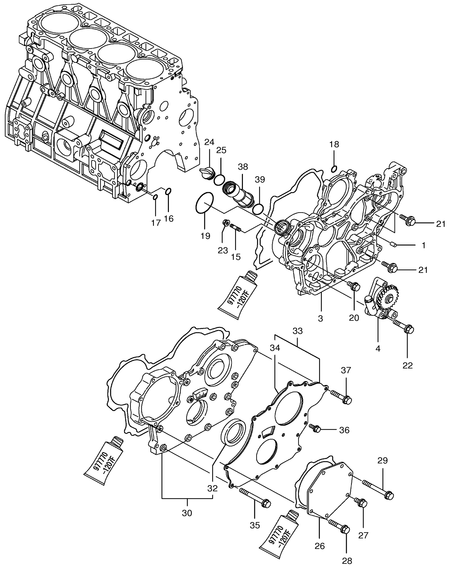
Fig. 012 GEAR HOUSING
