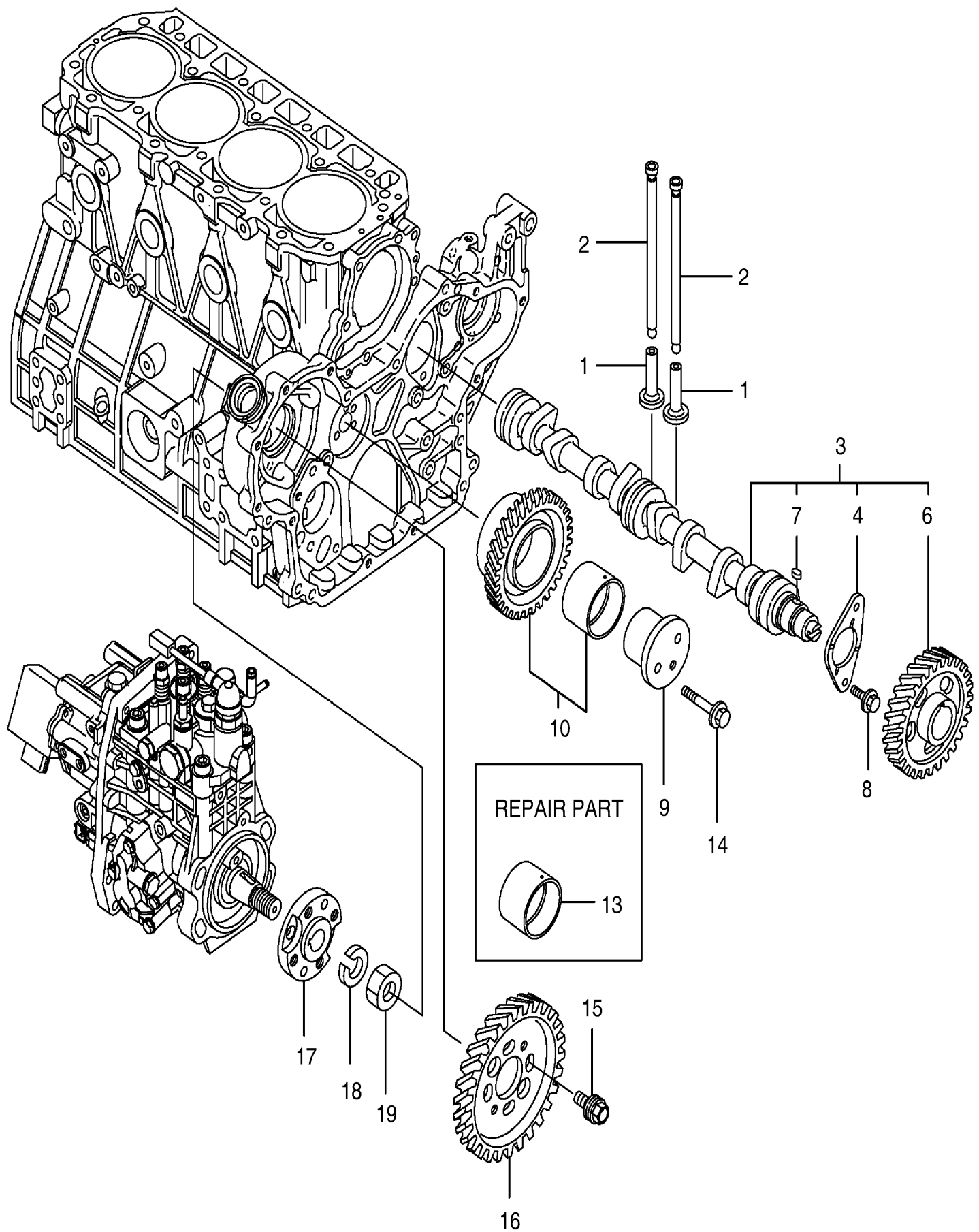
Fig. 017 CAM SHAFT & DRIVING GEAR
