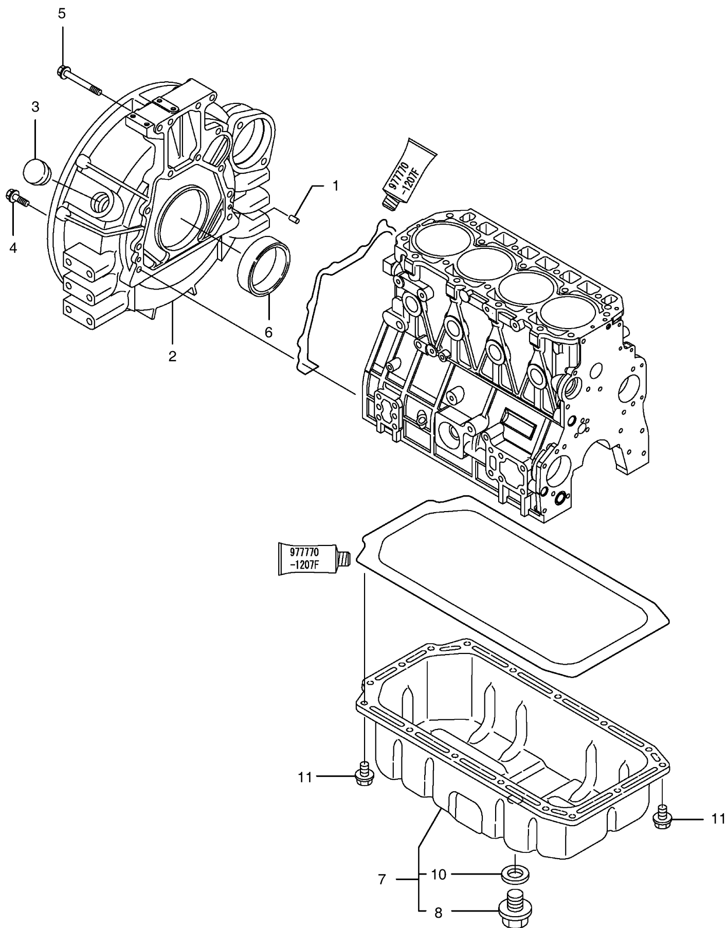
Fig. 013 FLYWHEEL HOUSING & OIL PAN
