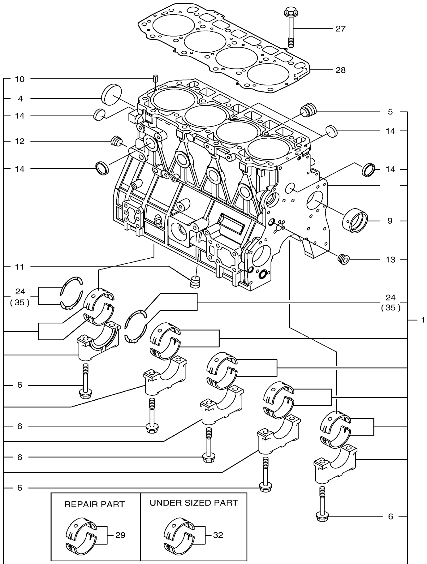
Fig. 011 CYLINDER BLOCK
