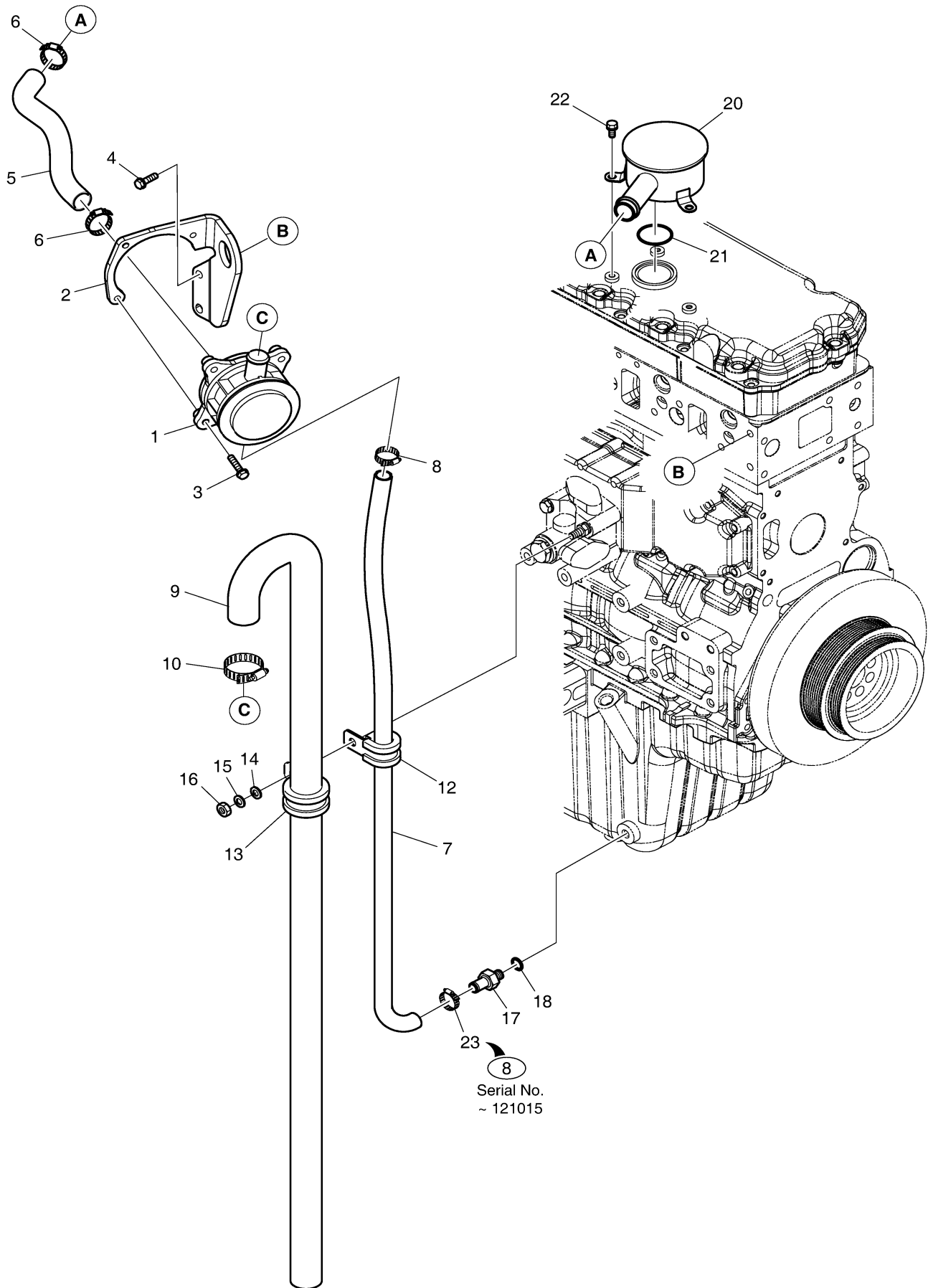
Fig. 015 BREATHER
