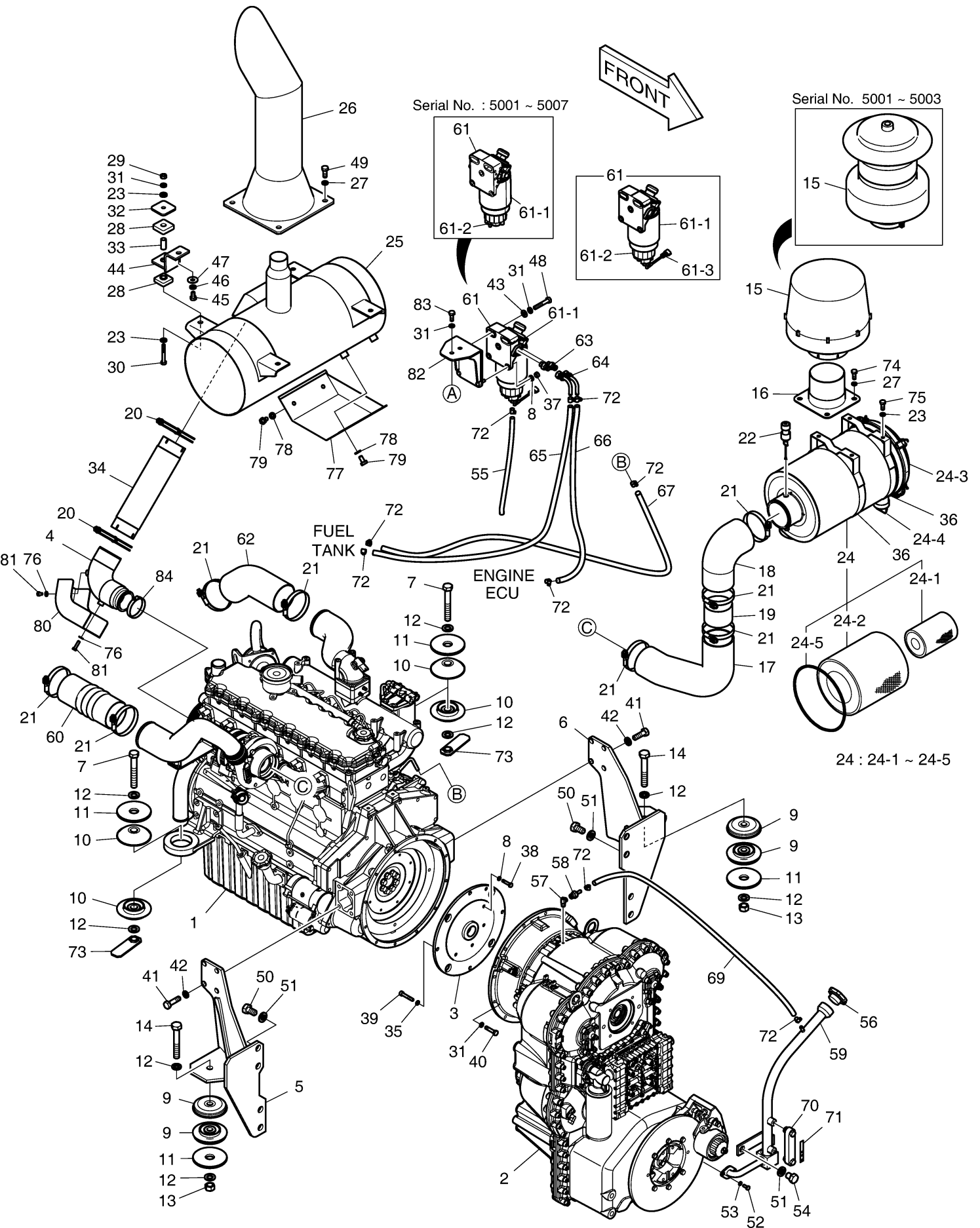
Fig. 1110 ENGINE MOUNTING
