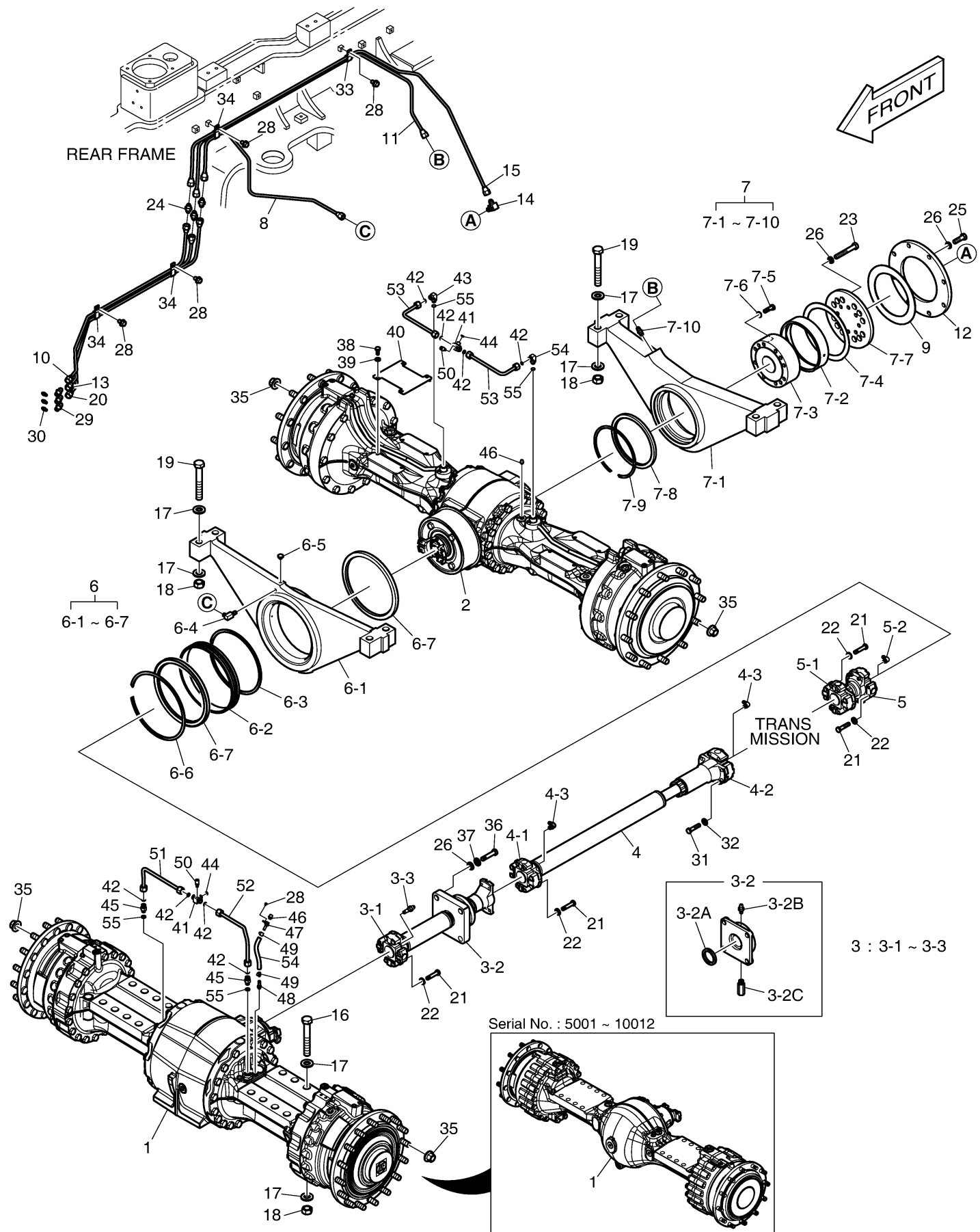
Fig. 1140 AXLE & DRIVE SHAFT
