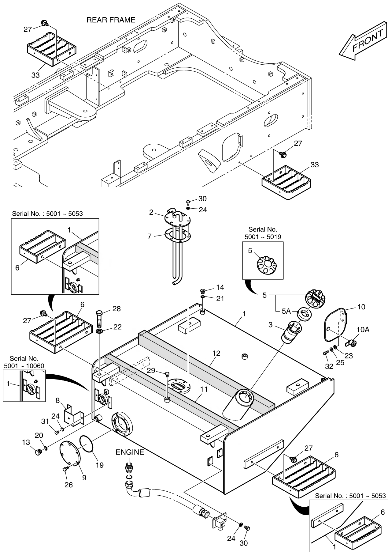
Fig. 1130 FUEL TANK
