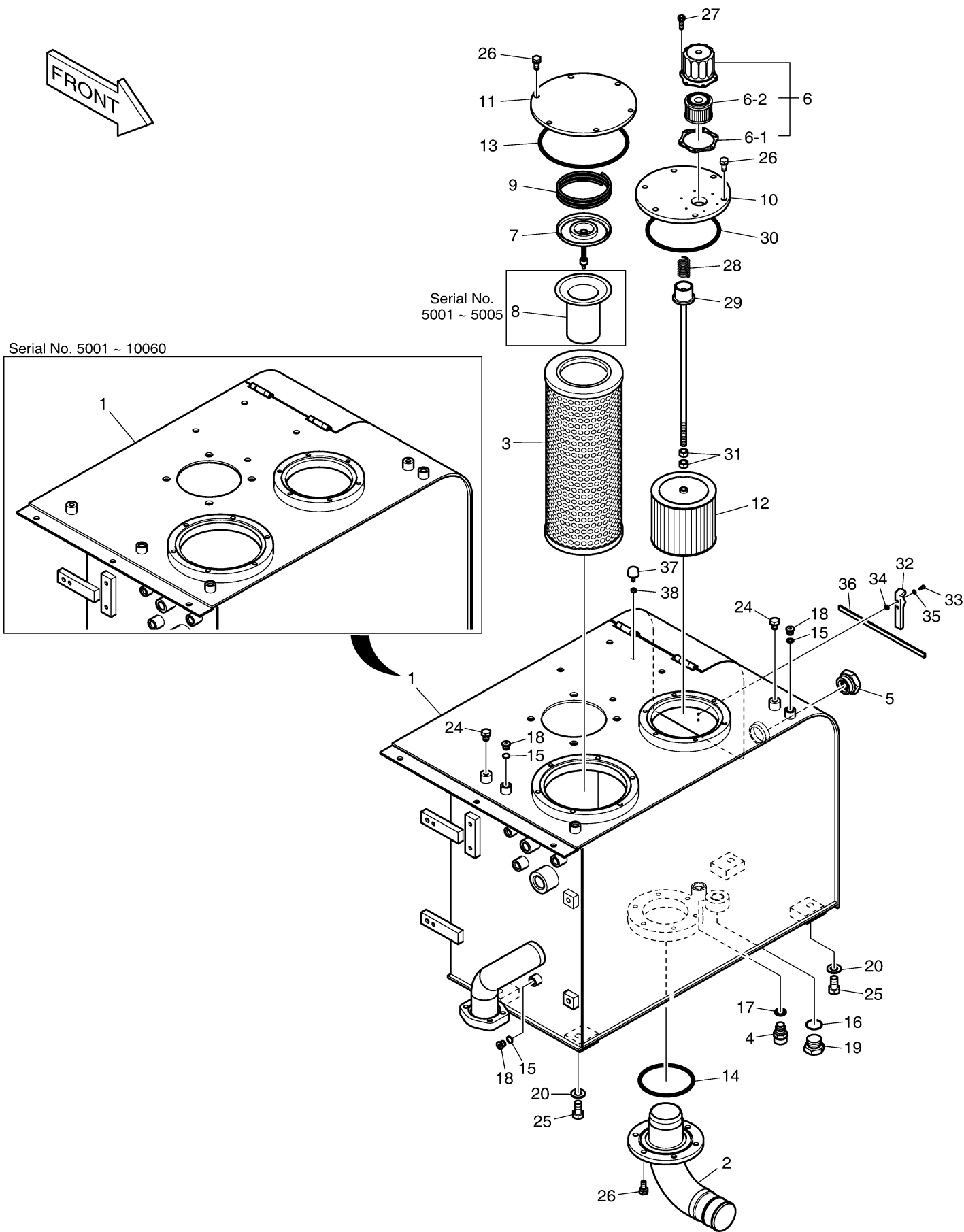
Fig. 1120 OIL TANK
