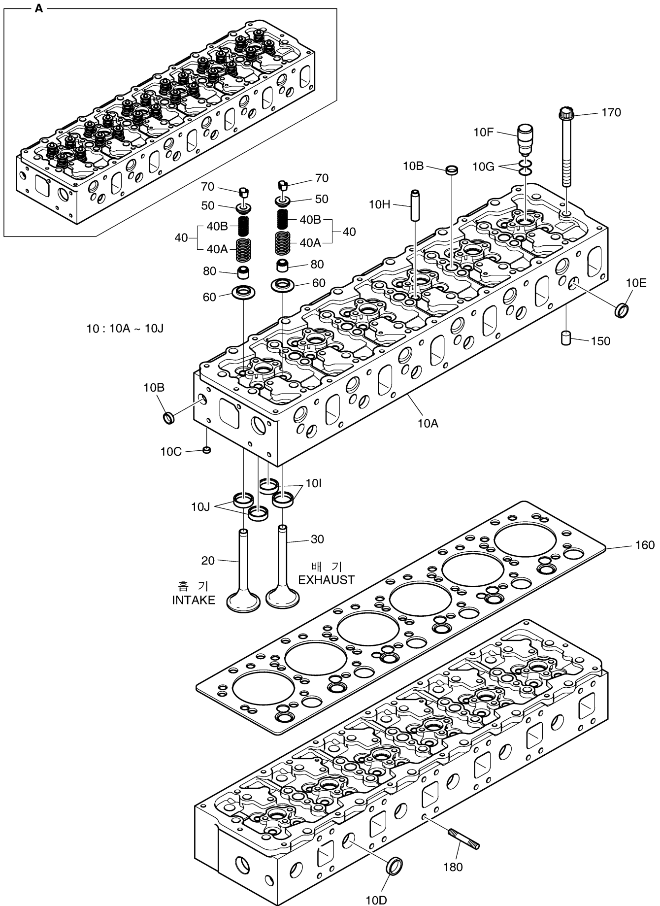
Fig. 007 CYLINDER HEAD
