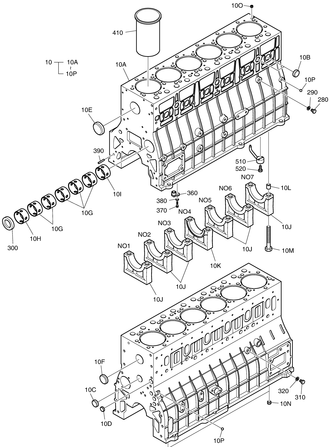
Fig. 001 CYLINDER BLOCK
