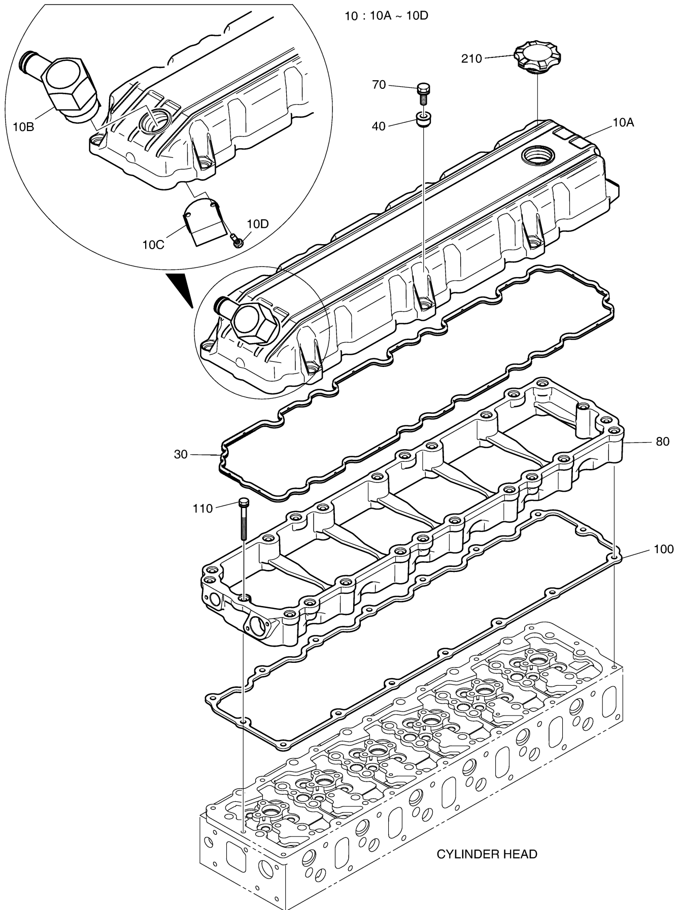
Fig. 008 CYLINDER HEAD COVER
