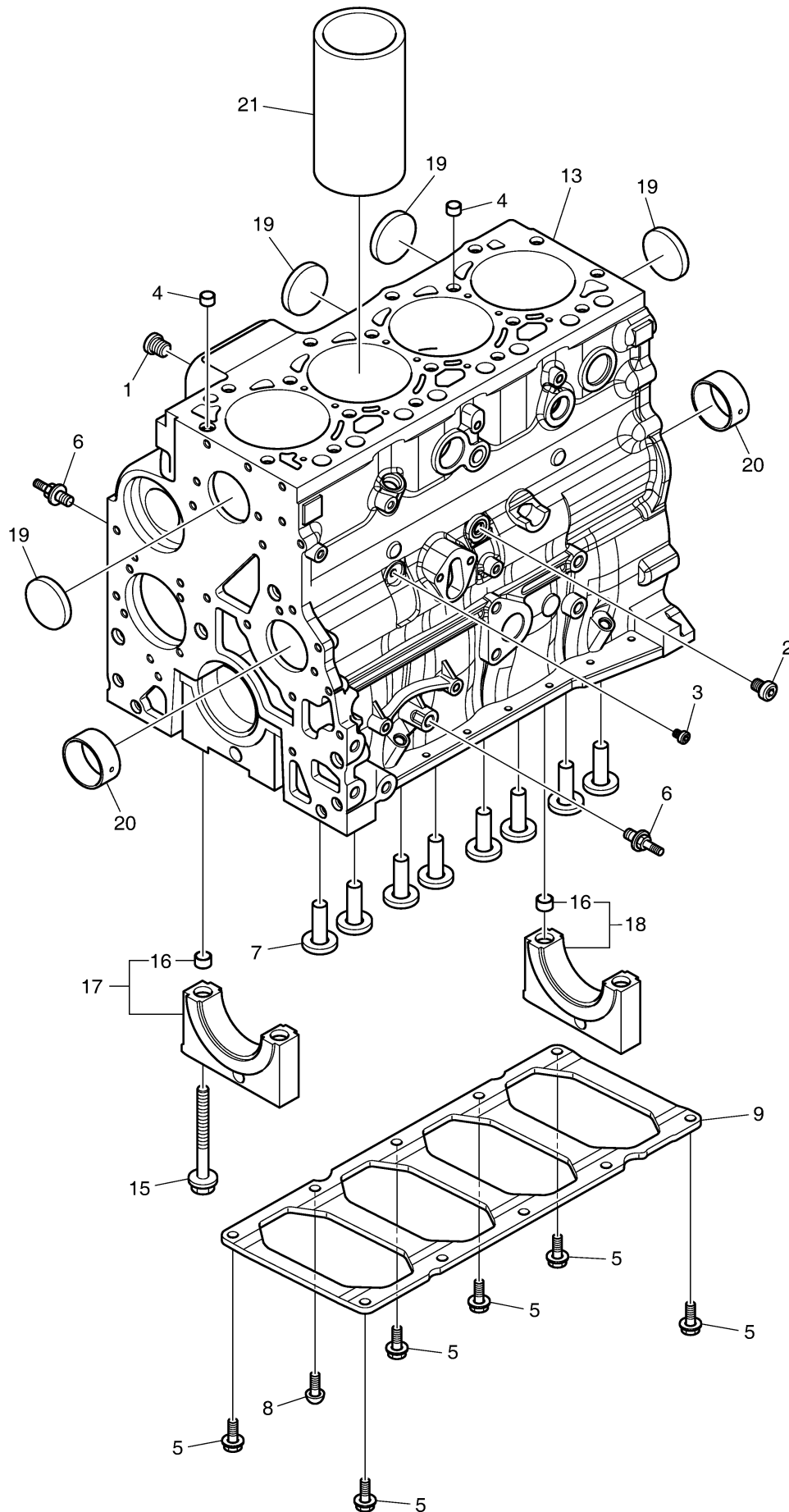
Fig. 013 CYLINDER BLOCK
