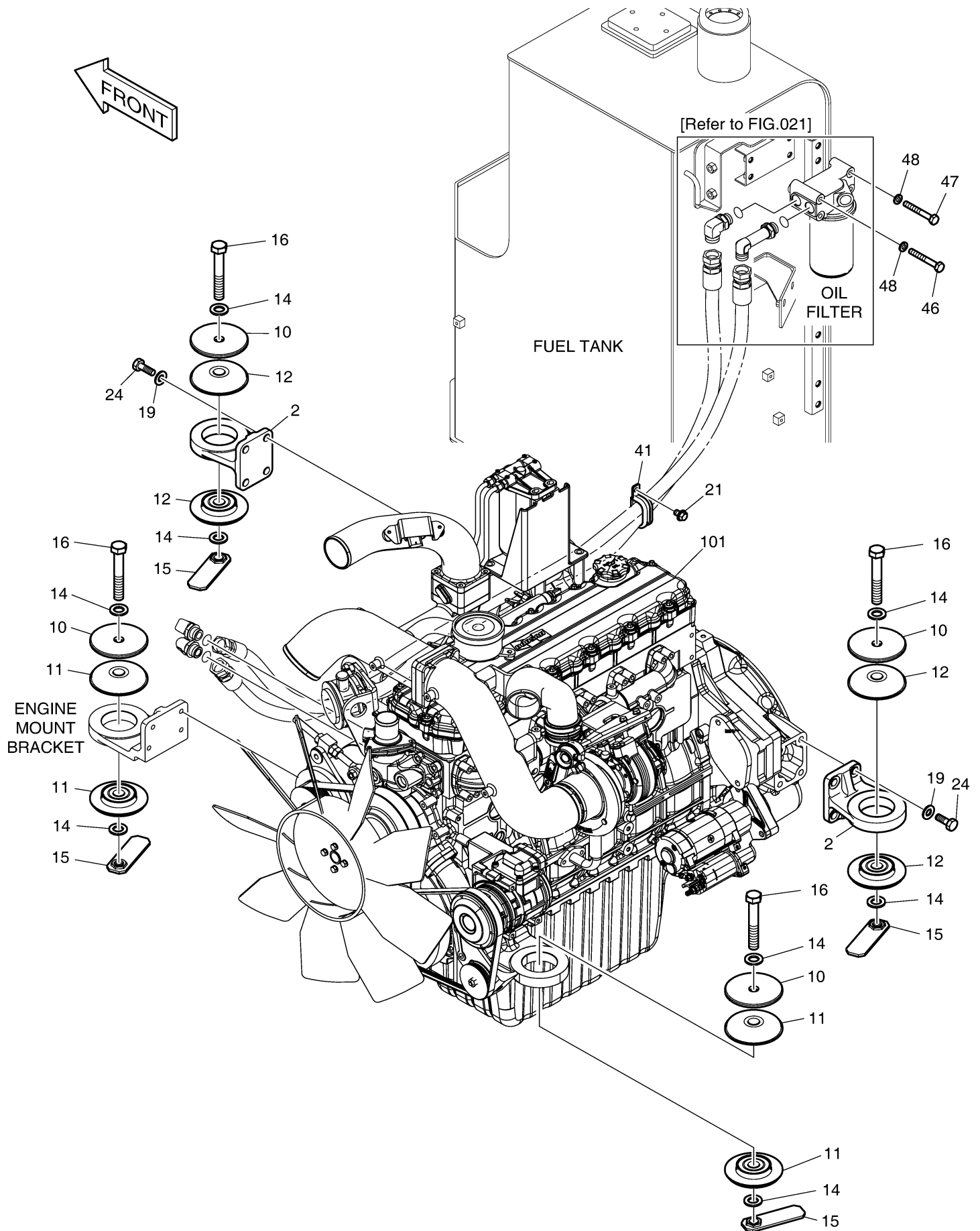
Fig. 1120 ENGINE MOUNTING
