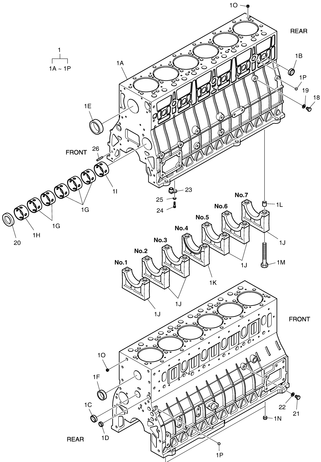
Fig. 001 CYLINDER BLOCK
