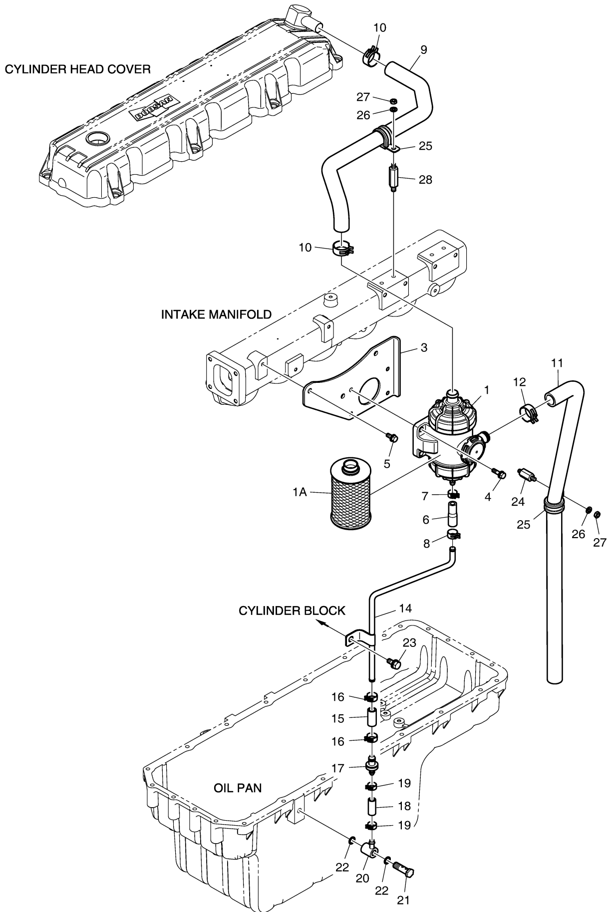
Fig. 007 BREATHER SYSTEM
