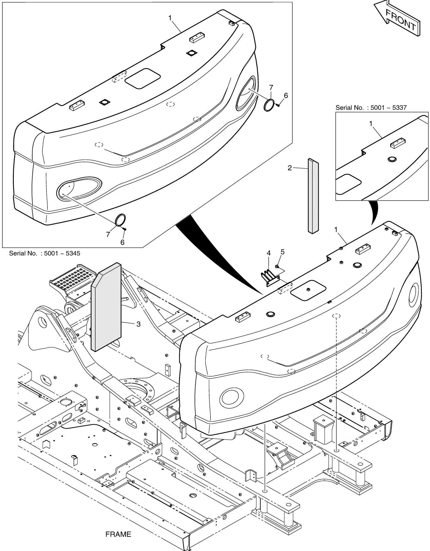
Fig. 1110 COUNTER WEIGHT
