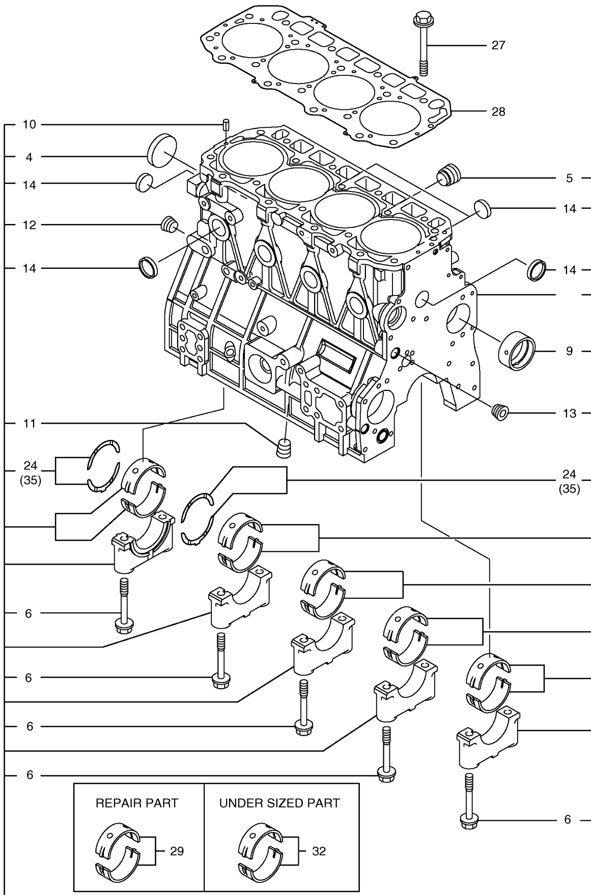
Fig. 011 CYLINDER BLOCK
