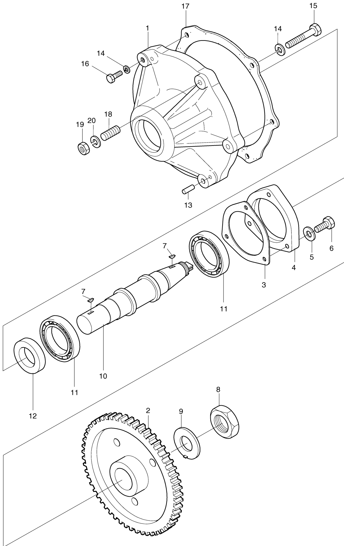
Fig. 013 BEARING CASE
