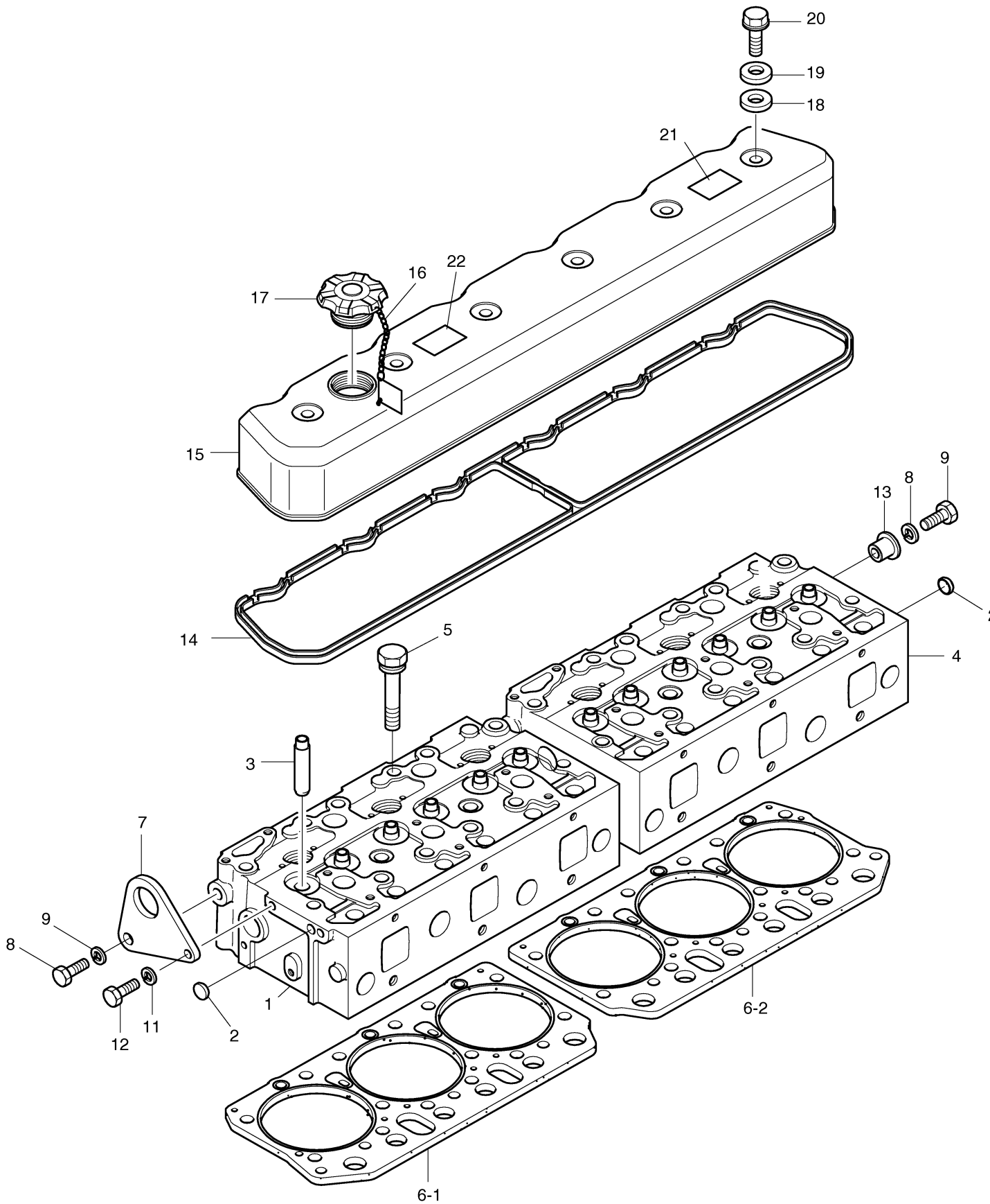
Fig. 017 CYLINDER HEAD
