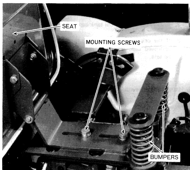
Figure 2 — Tractor Seat Adjustment
