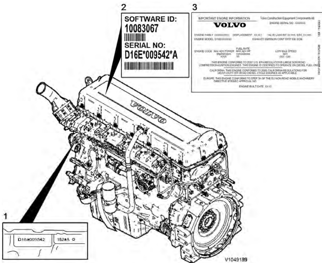
Figure 2 Engine identification, D16E
