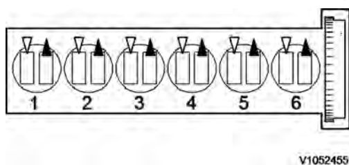
Figure 1 Cylinder numbering in relation to the flywheel
