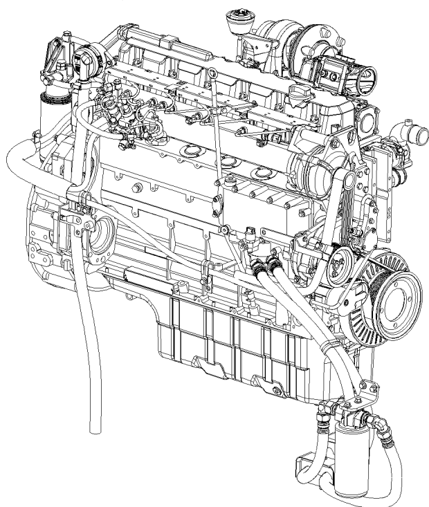
Figure 1 Engine, D7E
