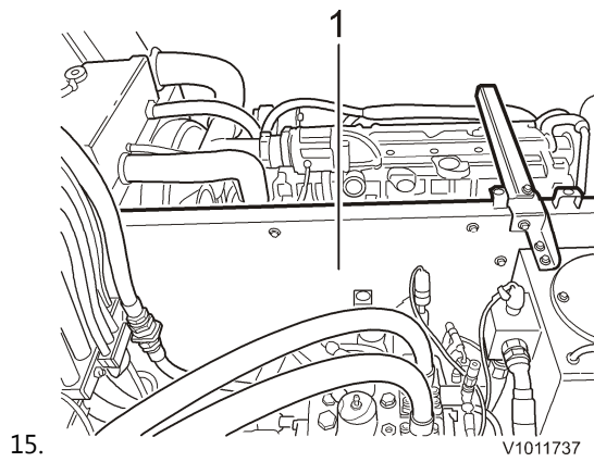
Figure 11 Engine/hydraulic compartment
