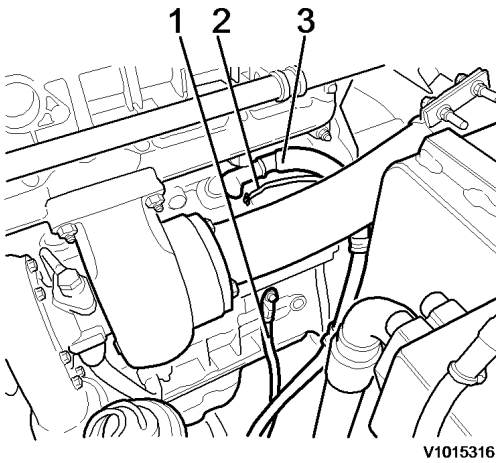
Figure 9 Engine/Starter motor
