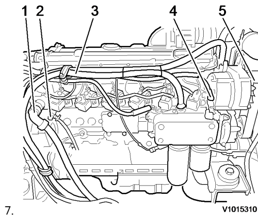
Figure 3 Engine, side view
