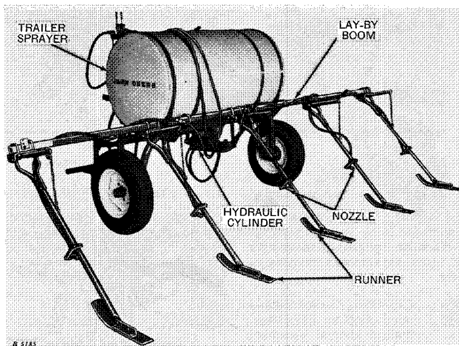
John Deere No. 2 Lay-By Boom Mounted on a Trailer Sprayer
