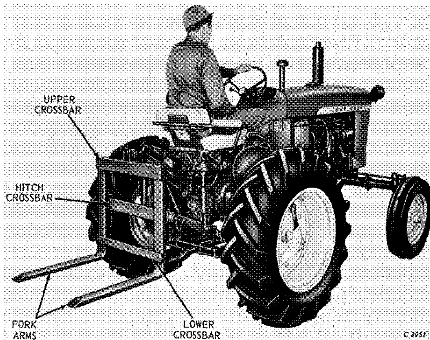
John Deere 26 Fork Lift Mounted on John Deere 1010 Tractor
