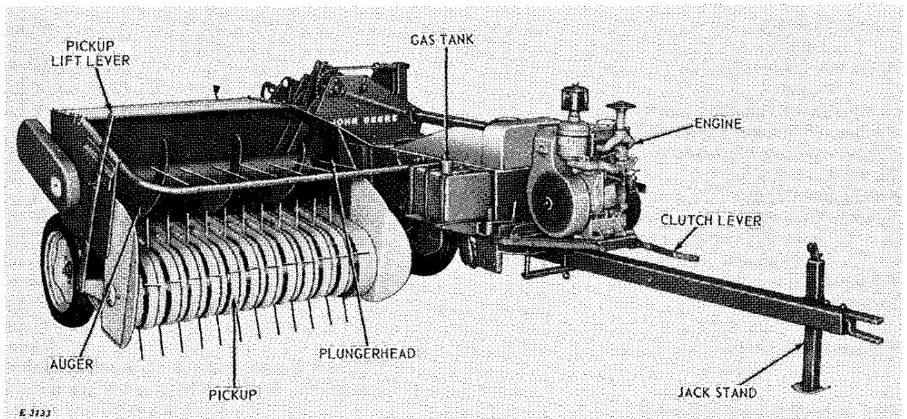
Right Front View—John Deere 24T Engine Baler
