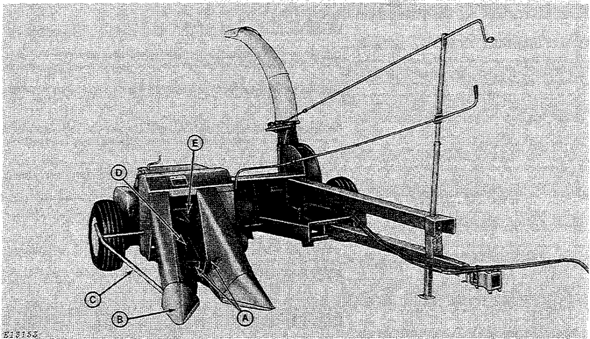
John Deere 35 Forage Harvester With One-Row Ear Corn Unit
