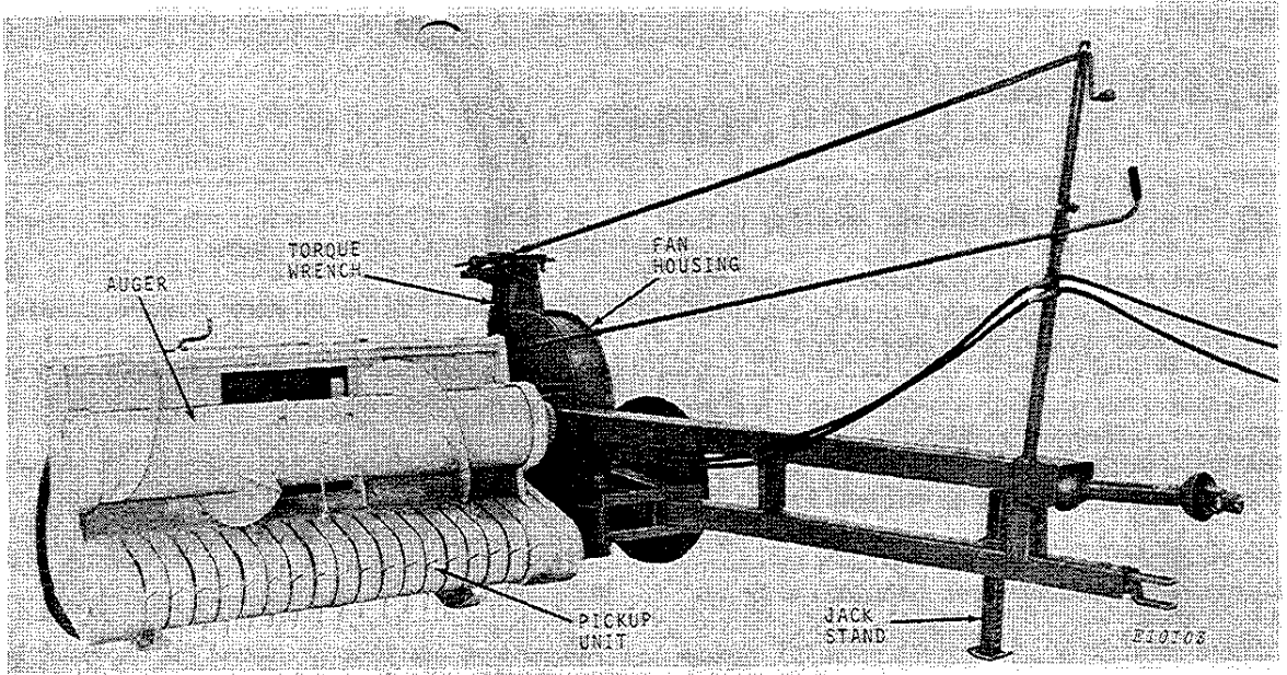
35 Forage Harvester with Pickup Unit
