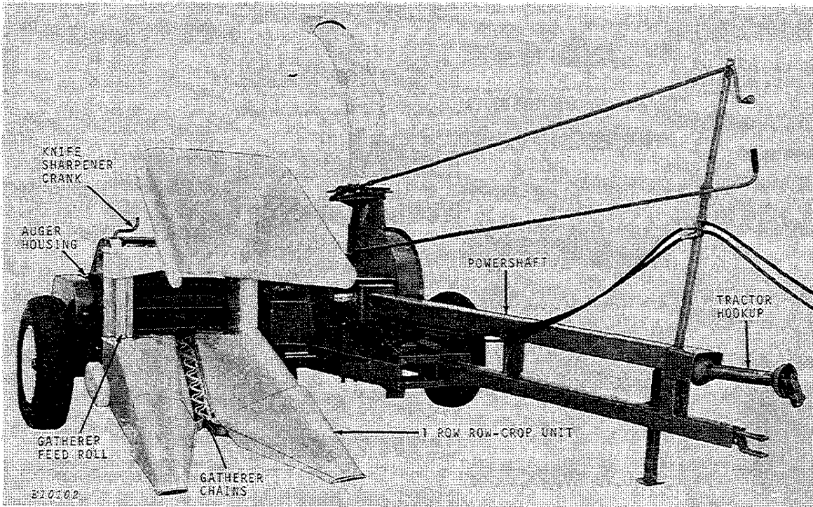
35 Forage Harvester with One Row Row-Crop Unit
