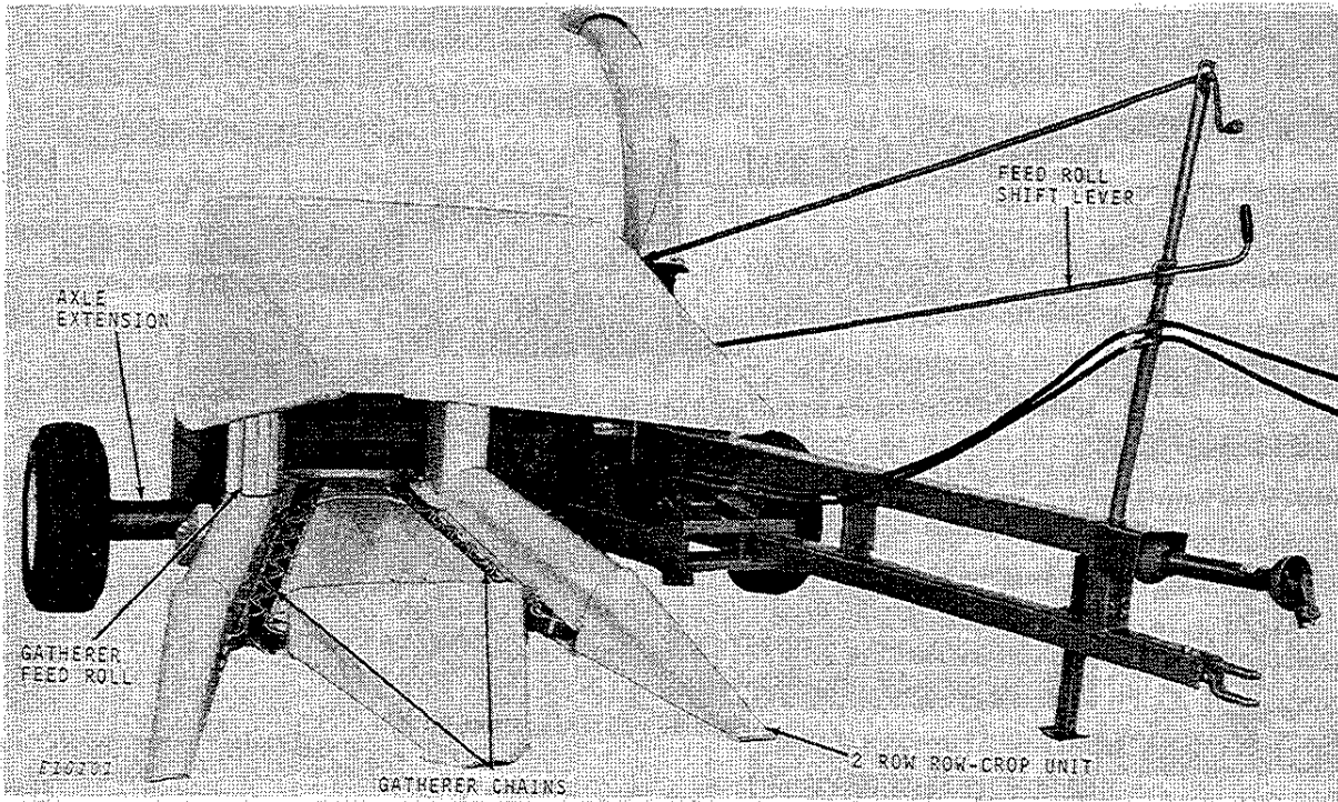
35 Forage Harvester with 30-Inch (76 cm) Two Row Row-Crop Unit
