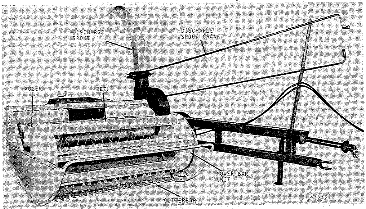
35 Forage Harvester with 6-Footer (1.83 m) Mower Bar Unit
