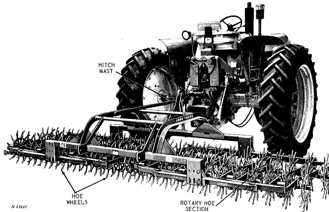
John Deere 642 Four-Section Flexible Rotary Hoe
