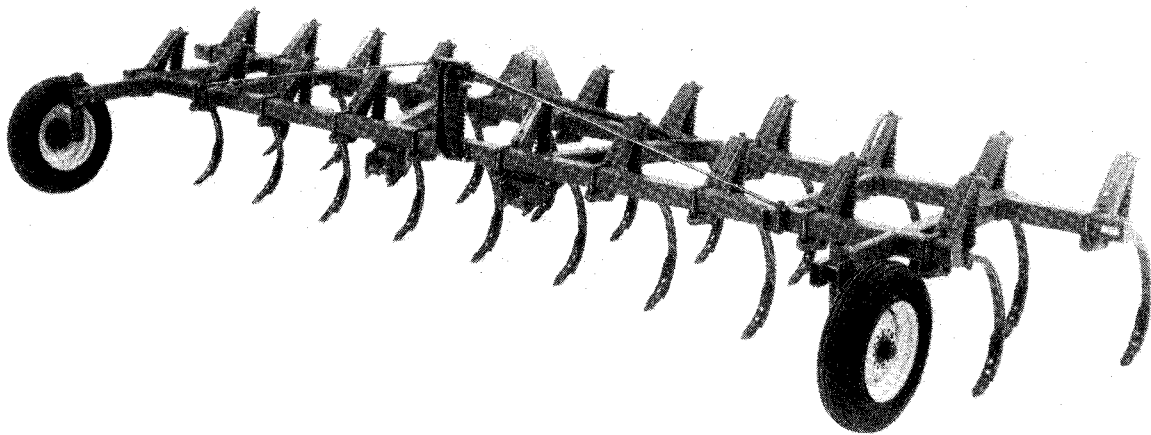
21-foot (6.4 m) 1610 Series 2-Bar Integral Chisel Plow
